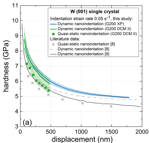
Figure 3: Indentation size effect of (001) W: (a) Hardness vs. displacement, and (b) Nix-Gao plot H^2 - 1/h . The blue and green lines represent the averaged hardness of the dynamic measurements using the G200 XP and DCM II. Results from the quasi-static indentation experiments are denoted by the green squares. The standard deviations are shown as blue- and green-shaded areas. Note, that the different size of the data sets, i.e. 20 for XP and 6 for each DCM II measurement series may cause differences in the standard deviations. The red line is the model prediction of the dynamic data. From the intercept with the ordinate, the H_0 is determined [11]. For comparison, hardness data of previously published studies [8, 9] have been added and are shown as grey lines and symbols.
