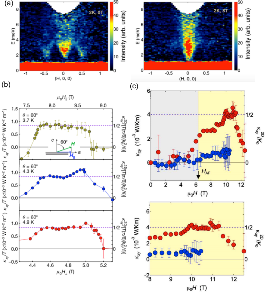
Figure 2.14: Key data of the Kitaev QSL candidate \alpha -RuCl 3 . (a) Inelastic neutron scattering was measured at T = 2 K along the reciprocal [H, 0, 0] (r.l.u.) direction in a zero external magnetic field and in a field of 8 T in the honeycomb plane, where the zigzag magnetic order was suppressed (taken from [90]), leaving only the continuum. (b) Half-integer thermal Hall conductance plateau: Half-integer thermal Hall conductance plateau was observed in the thermal Hall conductivity \kappa_{xy}/T in a field tilted at \theta = 60^\circ from ab plane plotted as a function of H_{\perp} . The top axes show the parallel field component, H_{\parallel} . The right scales represent the 2D thermal conductivity \kappa_{xy}^{2D}/T , in units of (\pi/6) (k_B^2/\hbar) . Violet dashed Hall conductivity represent the half-integer thermal Hall conductance \kappa_{xy}^{2D} / [T(\pi/6) (k_B^2/\hbar)] = 1/2 (taken from [91]). (c) Half-integer quantized anomalous thermal Hall: thermal Hall conductivity \kappa_{xy} in the antiferromagnetic (grey shaded area) and spin liquid (yellow) states for H \parallel a axis (red circles) and H \parallel b axis (blue circles) at 4.8 K. In the right axis, thermal Hall conductance per 2D layer \kappa_{xy}^{2D} is plotted in units of the quantum thermal conductance K_0 = (\pi^2/3) (k_B^2/h) T . The small but finite \kappa_{xy} experimentally observed for H \parallel b is likely attributed to a misalignment of the magnetic field direction from the b axis.
