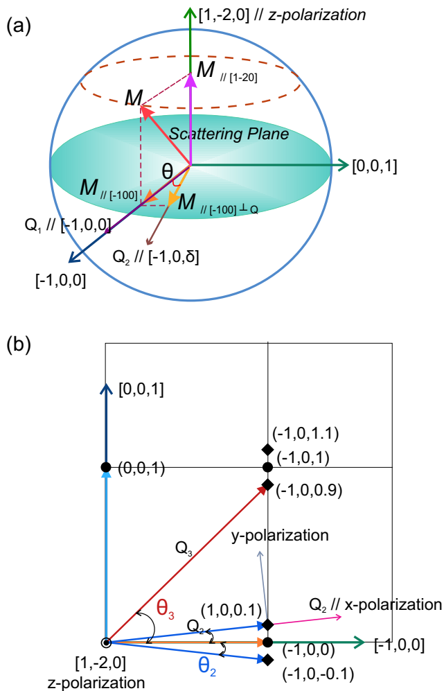
Figure 4.12: Scattering geometry of the experiments at DNS at MLZ. (a) The scattering plane is (h0l) plane where the magnetic moment \mathbf{M} in (hk0) plane can be decomposed into \mathbf{M}_{[1,-2,0]} and \mathbf{M}_{[\bar{1},0,0]} first. Then \mathbf{M}_{[\bar{1},0,0]} can be further projected onto [0,0,1] direction \mathbf{M}_{[\bar{1},0,0] \perp \mathbf{Q}} . \mathbf{Q}_1 is the scattering vector for the reflection [1,0,0] in crystallographic ab plane and \mathbf{Q}_2 is the scattering vector for modulated reflections. \theta is the angle between scattering vector \mathbf{Q} and (hk0) plane. (b) The (h0l) plane and the scattering vectors are depicted, where \theta is shown.
