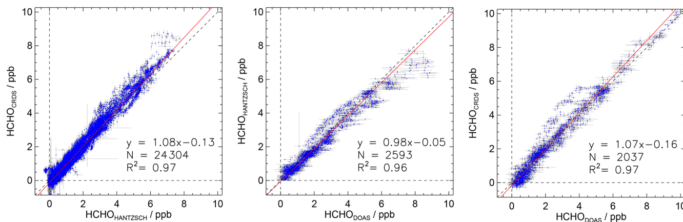
Figure 8. Correlation plots of measurements obtained by the Hantzsch, CRDS and DOAS instruments during experiments performed in the SAPHIR chamber. Data were acquired between June to December 2019 (time resolution: 180 s). Red lines show results from regression analysis. Error bars represent 1\sigma errors in the measurements.
