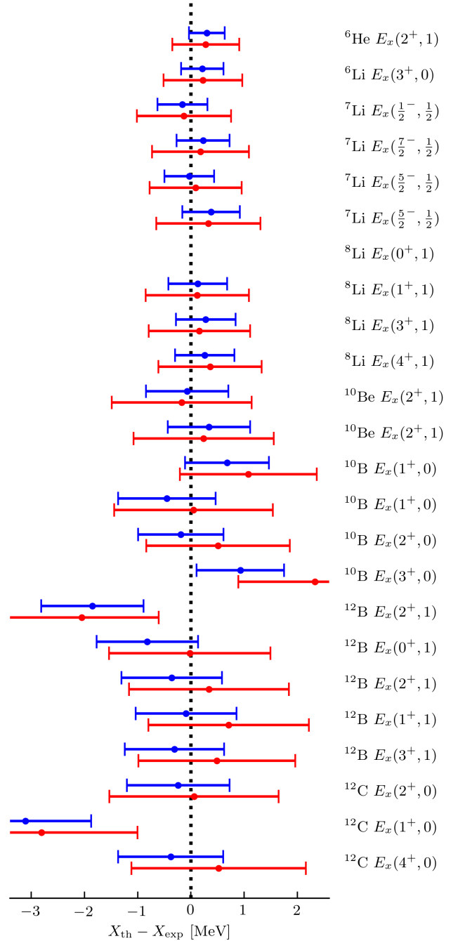
FIG. 13. (Color online) Central values (dots) for the difference of predicted (at \text{N}^2\text{LO} with 3NFs) and measured excitation energies from Tables III and IV, with 95% Bayesian confidence intervals (for truncation errors only) indicated as error bars. We omit the 0^+ in ^8\text{Li} because an experimental value is not available and note that the lowest 2^+ in ^{12}\text{B} is incorrectly predicted to be the ground state. For each excitation from the calculated ground state, the upper (blue) bar is for \Lambda = 450 MeV and the lower (red) bar is for \Lambda = 500 MeV. All results shown are for \alpha = 0.08 \text{ fm}^4 .
