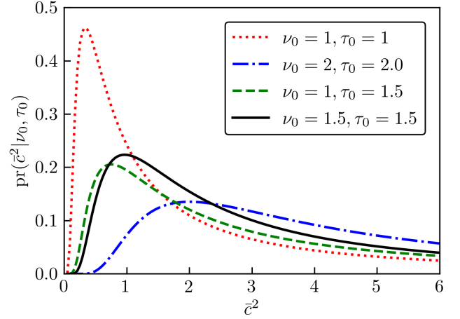
FIG. 12. (Color online) Prior pdf for the variance \bar{c}^2 of the expansion coefficient with several choices of hyperparameters \nu_0 and \tau_0 .
