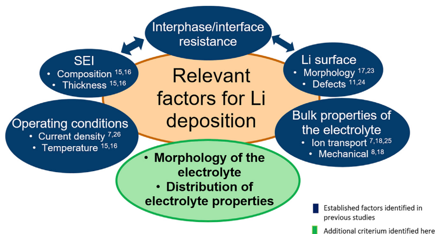
Figure 1. Critical parameters determining Li deposition behavior
