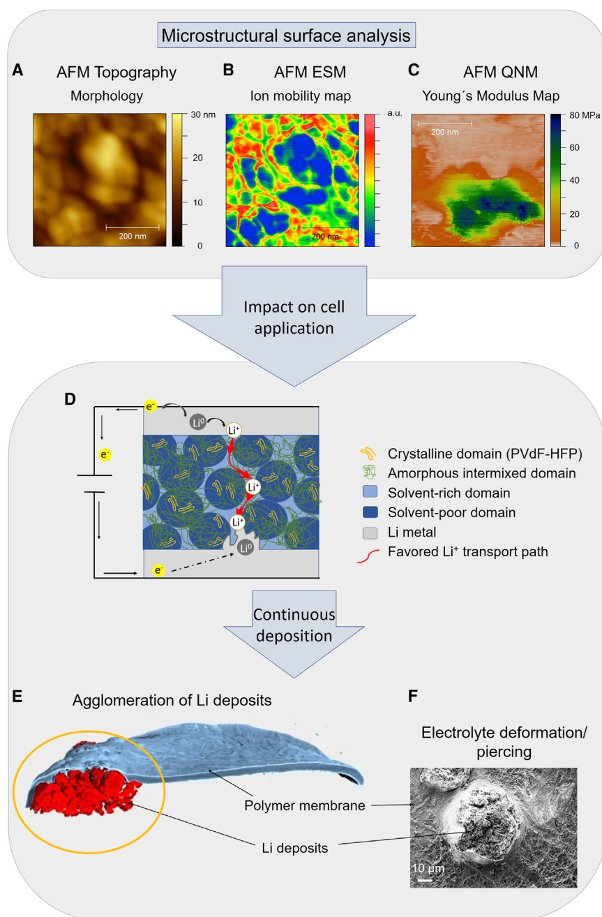
Figure 6. Schematic presentation of the Li deposition behavior
