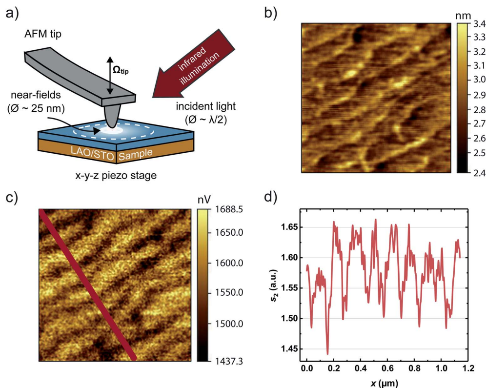
Fig. 4 (a) A sketch of the s-SNOM working principle is shown. (b) Shows the topography image of a 5 \mu\text{m} LAO/STO sample grown on a case [C] STO substrate with the corresponding optical image shown in (c). Both images are 1 \times 1 \mu\text{m} in size. From the same measurements, a single line profile of the optical signal is shown for the second order demodulation in (d).
