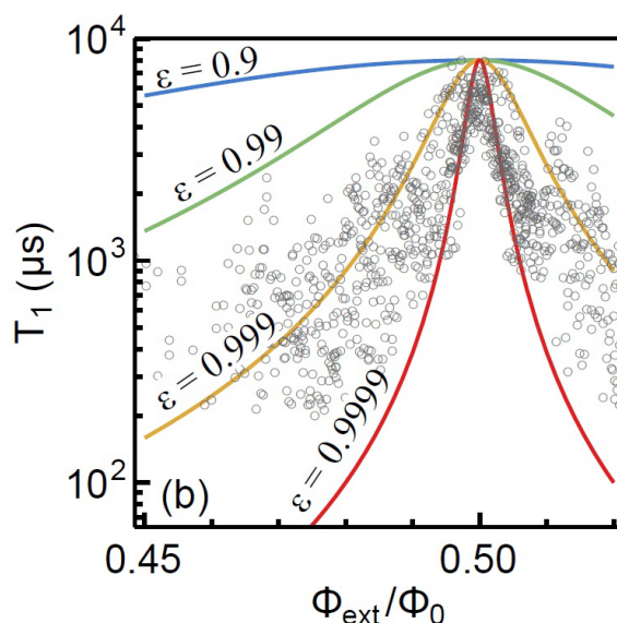
Figure 3: (from Ref. [15]) Empty circles: experimental data for T_1 at different values of external flux \Phi_{\text{ext}} . Solid lines: theoretical rates calculated from Eq. (80) with \text{Re}[Y_J] of Eq. (79), for a few values of \varepsilon and F chosen to bound the data at \Phi_{\text{ext}}/\Phi_0 = 1/2 .
