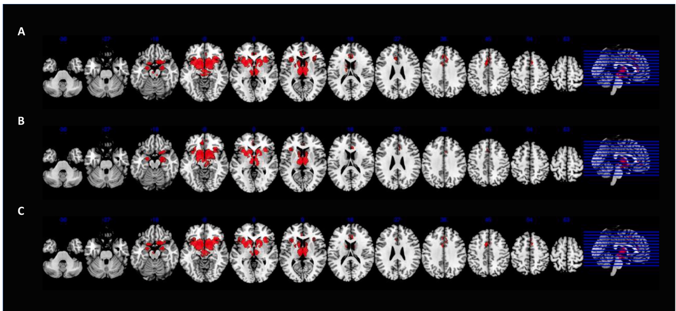
Fig. 4. Overview over the consensus connectivity networks (CCNs) derived from the clusters of our ALE meta-analysis on reward processing in ASD. Fig. 4A shows the CCN which used the right putamen - accumbens cluster from the TDC > ASD ALE as seed region. The CCN shows an extensive coactivation pattern, which is focused on the basal ganglia, thalamus, amygdala and insula, but also extends to the operculum, frontal orbital cortex and midbrain. It also includes the cingulate and paracingulate gyrus and the subcallosal cortex. The CCN which used the left hemispheric cluster in the left caudate, left accumbens and pregenual cortex from the TDC > ASD ALE as a seed region (Fig. 4B) shows a similar co-activation pattern as the former cluster. Fig. 4C depicts the CCN which used the right hemispheric putamen accumbens cluster from the ALE which pooled over all contrasts as a seed region. The CCN shows bilateral connectivity involving the basal ganglia, thalamus, insula, subcallosal, cingulate and paracingulate cortex, the frontal operculum, fronto-orbital cortex and the midbrain.
