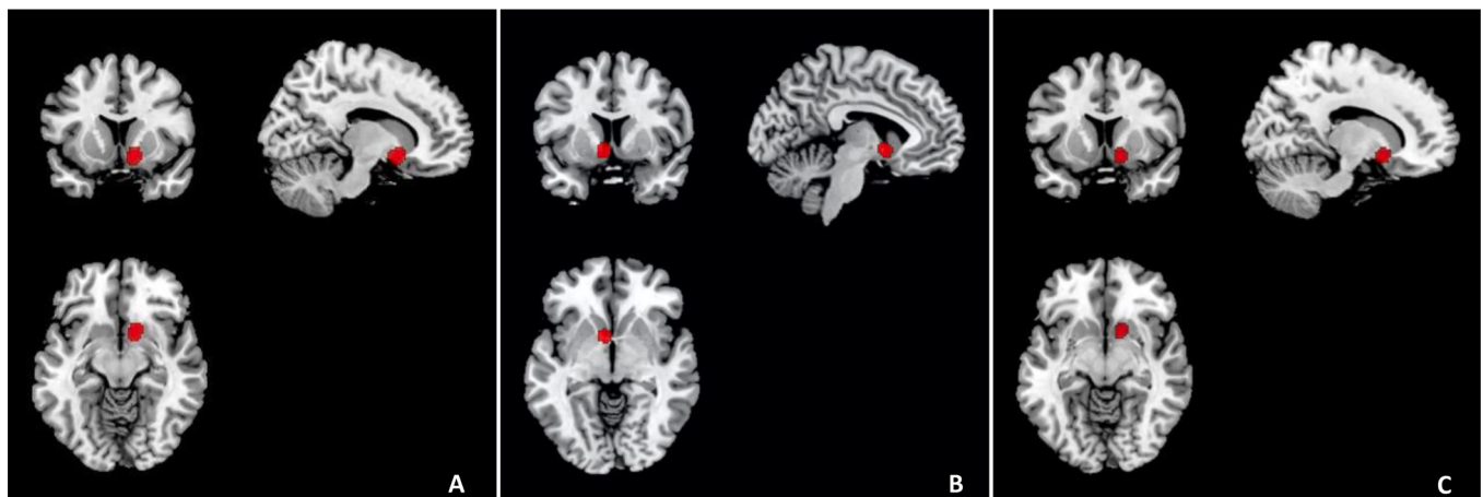
Fig. 2. Differential neural activations in ASD during reward processing. The ALE meta-analysis which only included hypoactivations resulted in two clusters. The larger of these was located in the right hemisphere centering around the right putamen and right accumbens with its fringes extending to the right caudate nucleus, the right fronto-orbital cortex and the subcallosal cortex (MNI peak coordinates: 12, 10, -10; 161 voxel) (A). The smaller of the two comprised the left accumbens, the left caudate nucleus, the pregenual area and the basal forebrain (MNI peak coordinates: -6, 6, -4; 98 voxel) (B). Pooling over all contrasts yielded a cluster which was located in the right putamen and right accumbens with its fringes extending to the right caudate nucleus, the fronto-orbital cortex and the subcallosal cortex (MNI peak coordinates: 12, 10, -10; 110 voxel) (C).
