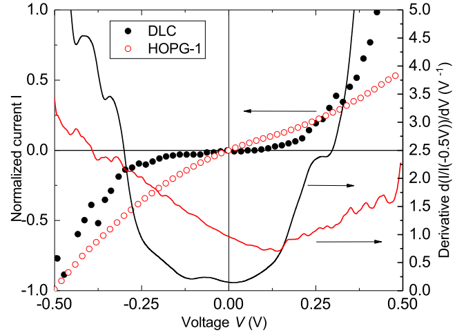
Fig. 9. TUNA results of the current-voltage characteristic curves (left y-axis) and their first derivatives (right y-axis) measured on a diamond-like carbon film (DLC) and on the position 1 of the bulk graphite surface of Fig. 1(a). The maximum current values used for normalization were: 59 pA (●) and 217 pA (○). The red line of the first derivative corresponds to the graphite sample and the black one to the DLC film. The derivatives were obtained from the normalized current data at -0.5 V.
