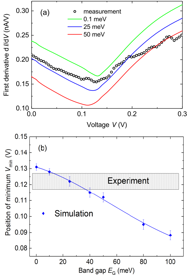
Fig. 5. (a) ( \circ ): First derivative of the tunnel current vs. applied voltage measured on the HOPG-Pd-1 sample shown in Fig. 1(a) and (lines) of the simulated tunnel currents at three different band gaps (0.1, 25, 50) meV with otherwise unchanged parameters. Note that the absolute values of the derivative are plotted. (b) Voltage position of the minimum of the first derivative vs. the band gap E_G . The ( \blacklozenge ) were obtained from the simulations. The line is only a guide to the eye. The range of the minimum in the first derivative of the experimental I - V curves of the HOPG-1 sample is given by the shadowed rectangular region.
