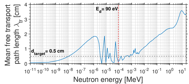
Fig. 9: Mean free transport path length \lambda_{tr} of neutrons inside the tantalum target. At kinetic energies greater than the displacement threshold E_d the average path length mostly exceeds the target thickness, resulting in rare interaction events.
