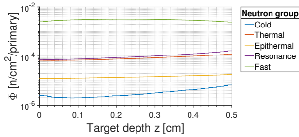
Fig. 7: Neutron fluence \Phi for 5 different neutron energy groups according to table 2 obtained with a PE moderator. The number of neutrons decreases with decreasing neutron energy.
