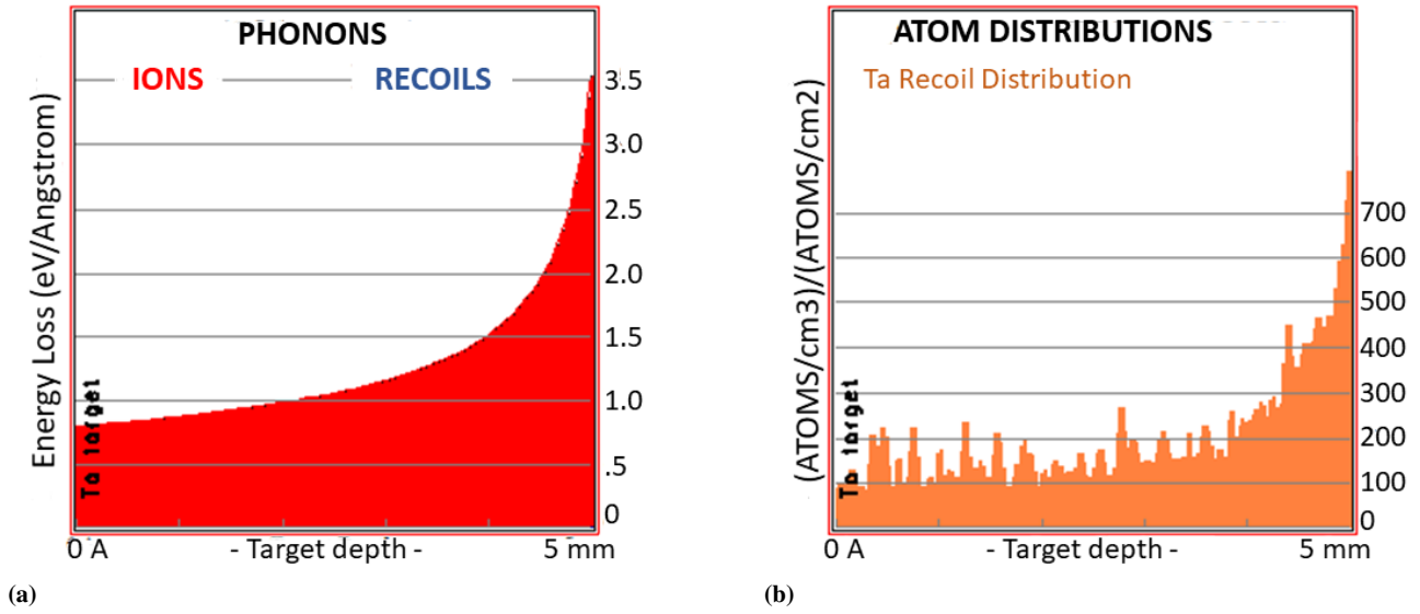
Fig. 2: Proton electronic energy deposition along the target depth and recoil atom distribution in SRIM. (a) The protons deposit more and more energy with increasing target depth, the maximum (Bragg peak) is not located in the target. Recoils are not depicted, as the corresponding IONIZ.txt file revealed their electronic energy losses to be \sim 4 orders of magnitude smaller. Indeed, they lose a significant amount of energy by phonon production (see Fig. 1b). (b) Distribution of Ta recoil atoms produced along the target depth. The highest recoil density at the rear implies that besides inelastic energy losses, also the nuclear deposited energy peaks at the rear, and hence the number of atomic displacements.
