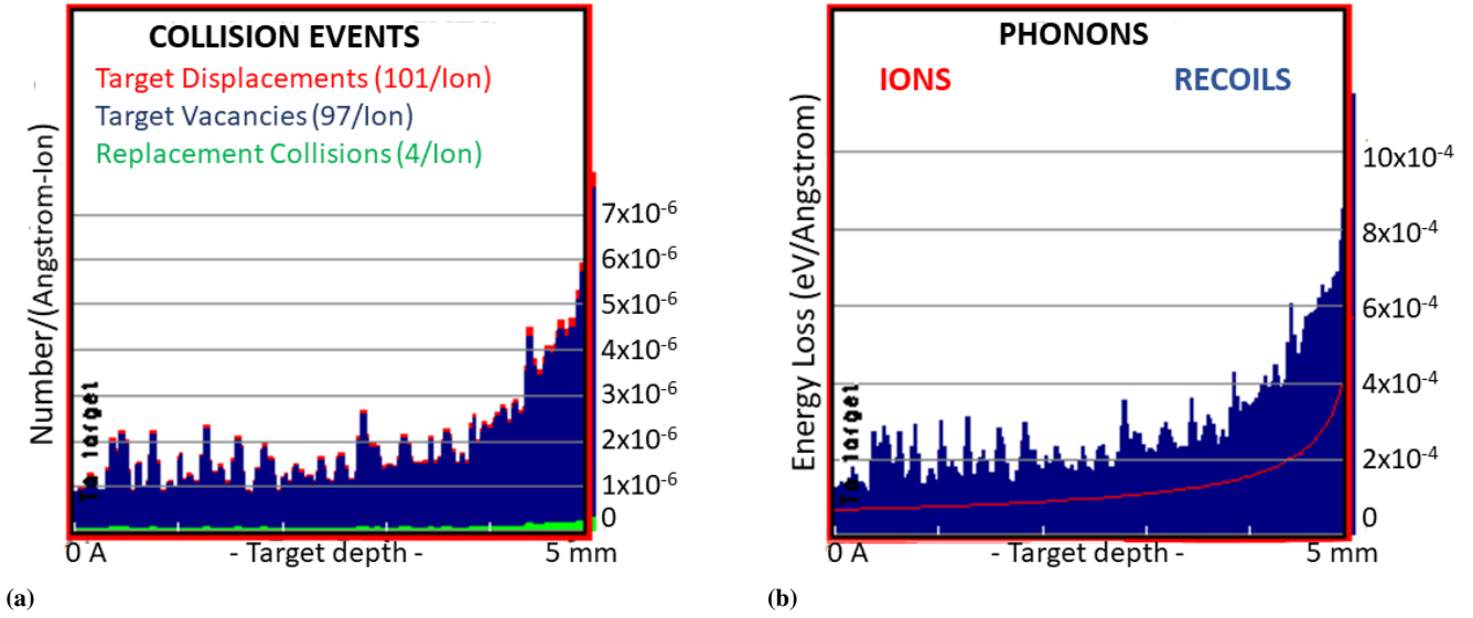
Fig. 1: SRIM simulation of different collision events and phonon production in the tantalum target. (a) Calculations for the damage rates R_d are based on the number of target displacements, i.e. 101/Ion in the case of an average and \sim 8 \times 10^{-6} \text{ \AA}^{-1} \text{ Ion}^{-1} for a peak value. Note that the numbers of events are related as: n(\text{Target Displacements}) = n(\text{Target Vacancies}) + n(\text{Replacement Collisions}) . Furthermore: n(\text{Target Displacements}) > n(\text{Target Vacancies}) > n(\text{Replacement Collisions}) . (b) Ta recoil atoms spend most of their energy for phonon production. Note, that the generated PHONON.txt file revealed the ordinate unit to be \text{eV \AA}^{-1} \text{ Ion}^{-1} instead of \text{eV \AA}^{-1} .
