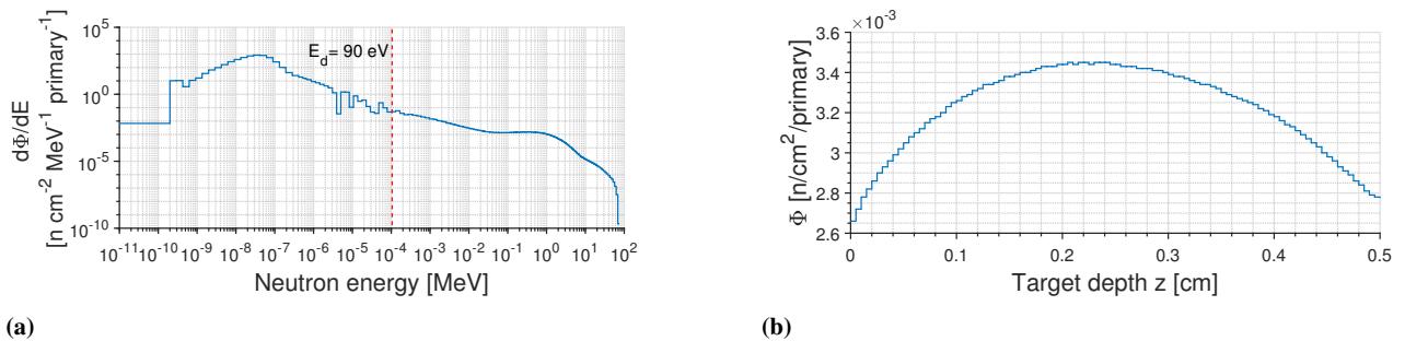
Fig. 6: Neutron spectral data for a PE moderator and 70 MeV primary proton energy. (a) Energy differential neutron spectrum obtained with a USRTRACK card. The thermal peak results from the spherical moderator and might seem to be overemphasized, which is a consequence of the fixed bin width of the 260 FLUKA neutron energy groups below 20 MeV. (b) Neutron fluence \Phi over the target depth obtained with a USRBIN card. The neutron density peaks at the middle of the target and decreases towards the outer surfaces.
