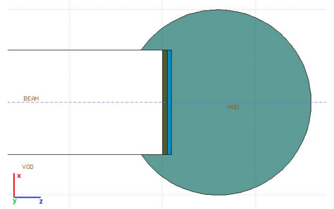
Fig. 3: FLUKA geometry taken from flair [56, 57], modified with coordinate axes. The proton beam impinges from the left perpendicular on the target (dark green), the emitted neutrons get thermalized in the spherical PE moderator (light green) beyond a beamstop (blue).
