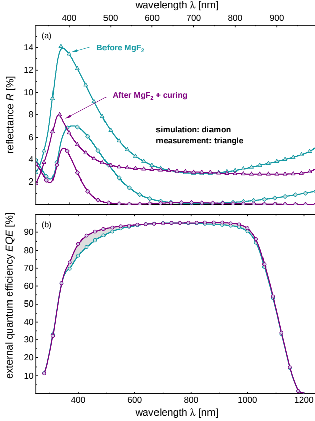
Figure 6.17.: Optical and electro-optical effects of an MgF 2 ARC on TPC solar cells. (a) Simulated (diamonds) and measured (triangles) reflectance for the front side contact of c-Si/SiO 2 /μc-SiC:H(n)/ITO with and without MgF 2 as a function of the wavelength. (b) External quantum efficiency (EQE) with and without MgF 2 ARC as a function of the wavelength. MgF 2 reduces the reflection in the long and in the short wavelength range, which improves the EQE in these regions and results in a higher J_{sc} . Data in this figure was originally published in [9] (CC BY 4.0) and adapted.
