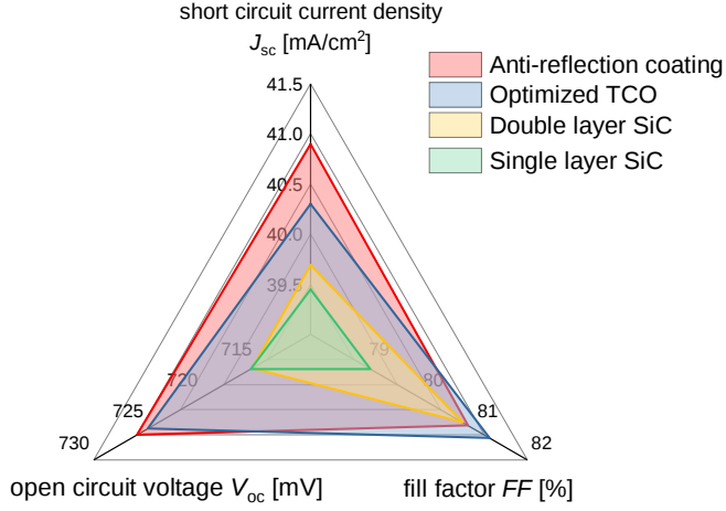
Figure 0.1.: Evolution of the solar cell parameters J_{sc} , V_{oc} and FF using a single layer \mu\text{c-SiC:H}(n) (green, power conversion efficiency \eta = 22.3\% ), a double layer of \mu\text{c-SiC:H}(n) (yellow, \eta = 22.9\% ), an optimized TCO deposition (blue, \eta = 23.8\% ) and an anti-reflection coating (red, \eta = 24\% ).
