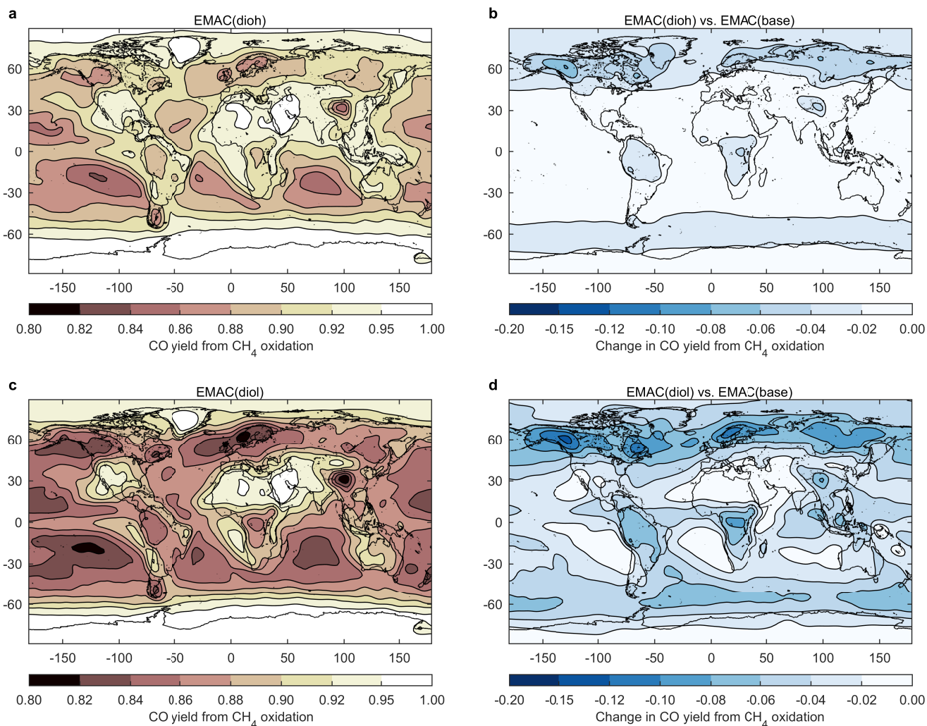
Extended Data Fig. 9 | Effect of cloud processing on modelled carbon monoxide. a–d , Yield of CO originating from methane (CH 4 ) oxidation modelled by EMAC (dioh) ( a ) and EMAC (diols) ( c ), and change in CO yield from CH 4
