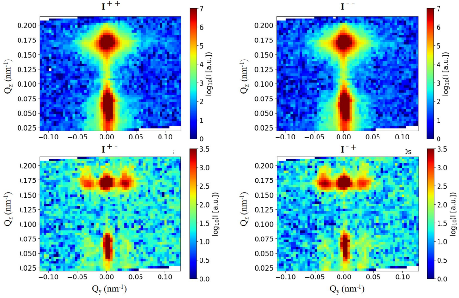
Figure 9.17: Q_y - Q_z -maps of the four different GISANS channels measured at T_B = (5.60 \pm 0.02) K on \text{SF}_{\text{high}}(2) after subtraction of a rotation angle of 4.7^\circ .
