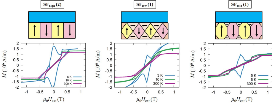
Figure 6.2: M(H_{\text{ext},\perp}) of \text{SF}_{\text{high}}(2) , \text{SF}_{\text{low}}(1) and \text{SF}_{\text{mid}}(1) measured below and above T_c in an out-of-plane applied magnetic field, adapted from the supplementary information in [181].
