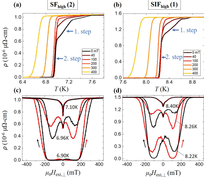
Figure 6.6: (a,b) \rho(T) in a constant out-of-plane applied field, for \text{SF}_{\text{high}}(2) and \text{SIF}_{\text{high}}(1) , respectively. (c) \rho(H_{\text{ext},\perp}) at constant temperature for \text{SF}_{\text{high}}(2) and for the reference sample \text{SIF}_{\text{high}}(1) (d).
