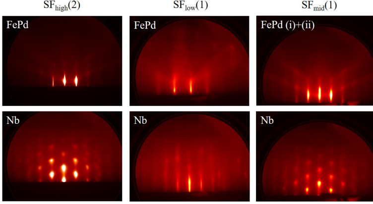
Figure 5.6: RHEED measurements taken at room temperature after the growth of the FePd layers (top) and the Nb layers (bottom) of samples SF_{\text{high}}(2) , SF_{\text{low}}(1) , and SF_{\text{mid}}(1) .
