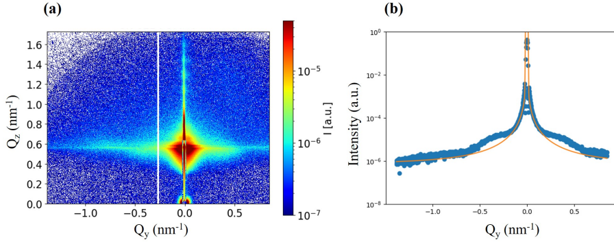
Figure 9.18: (a) Q_y - Q_z -map of GISAXS measured at room temperature on \text{SF}_{\text{high}}(2) and (b) corresponding I(Q_y) at the specular line.
