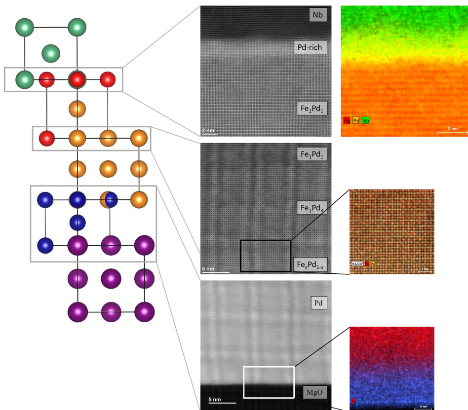
Figure 9.4: Sample stack of S/F samples (left) and HAADF-STEM measurements of SF_{low}(1) (middle). The high substrate temperature of SF_{high} with T_s = 820 K has led to an interdiffusion of the FePd and Pd layers. Nearly defect-free Pd is grown in the vicinity of MgO which subsequently mixes with Pd; forming first a Fe_xPd_{1-x} layer with a small amount of Fe; and in a second step a Fe_1Pd_3 layer, which can be revealed by the STEM-EDX elemental map on the right. Near the FePd/Nb interface, the L1_0 -ordered phase of Fe_1Pd_1 is established. Colors are indicated in the legend.
