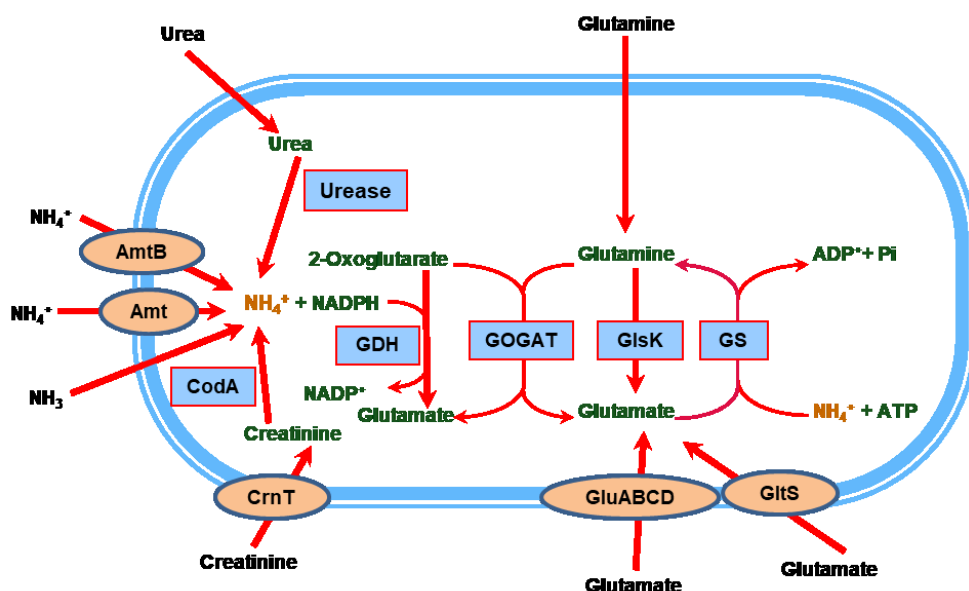
Fig. 1 Nitrogen metabolism in C. glutamicum . Rectangular boxes: enzymes, round boxes: importers. Amt, AmtB: ammonium uptake system; GluABCD: glutamate uptake system; GDH: 8
