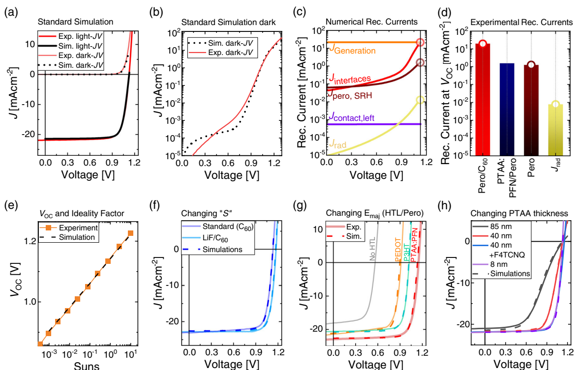
Figure 1. a,b) Experimental and numerically simulated light and dark JV curves of p–i–n-type cells based on PTAA/PFN-Br/triple-cation perovskite/ C_{60} in a linear and logarithmic representation. The interface recombination velocities and bulk lifetime were obtained from TRPL measurements. [22] c) Simulated voltage-dependent radiative and nonradiative recombination currents in the neat perovskite and at both interfaces compared to the generation current. Interfacial recombination reduces the possible open-circuit voltage, which is roughly 10× larger than Shockley–Read–Hall recombination in the neat material. [50] d) This is consistent with experimentally measured recombination currents under open-circuit conditions using steady-state PL measurements. [50] e) The simulation parameter set also reproduces the ideality factor ( n_{\text{ID}} \approx 1.35 ) of the standard cells. [78] The standard simulation settings allow us to fit several experimental results by changing a single parameter depending on the particular experiment. f) Inserting LiF between the perovskite and C_{60} leads to concurrent increase of the TRPL lifetime, device V_{\text{OC}} , and PCEs above 21%. [22] The TRPL results suggest that S decreases by one order of magnitude upon application of LiF, which allows us to reproduce the experimentally observed V_{\text{OC}} gain of 35 mV. g) Cells with different HTLs and varying majority carrier band offsets as obtained from ultraviolet photoelectron spectroscopy (UPS) measurements. [50] Implementing energy offsets at the p-interface for the cells with a poly(3,4-ethylenedioxythiophene) polystyrene sulfonate (PEDOT:PSS) and poly(3-hexylthiophen-2,5-diyl) (P3HT) hole transport layer allows us to reproduce the experimental JV curves. h) Cells with changing PTAA thickness. The mobility in the PTAA layer has a significant impact on the device FF consistent with previous work. [79] The fitting allowed us to fine-tune the perovskite and the PTAA layer mobility ( \mu_{\text{perov}} = 1 \text{ cm}^2 \text{ V}^{-1} \text{ s}^{-1} , \mu_{\text{PTAA}} = 1.5 \times 10^{-4} \text{ cm}^2 \text{ V}^{-1} \text{ s}^{-1} , while \mu_{C_{60}} = 1.0 \times 10^{-2} \text{ cm}^2 \text{ V}^{-1} \text{ s}^{-1} ).
