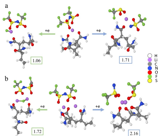
Figure 4. a) Reduction potentials (in Volts) vs. \text{Li}|\text{Li}^+ of \text{LiTFSI} -PAM with the SMD(acetone)/M052X/6–31 + G(d,p) model chemistry highlighting defluorination (left) and S–N cleavage (right). b) Reduction potentials vs. \text{Li}|\text{Li}^+ of \text{Li}_2\text{TFSI} -PAM (simulating salt aggregation) with the SMD(acetone)/M052X/6–31 + G(d,p) model chemistry highlighting defluorination (left) and S–N cleavage (right).
