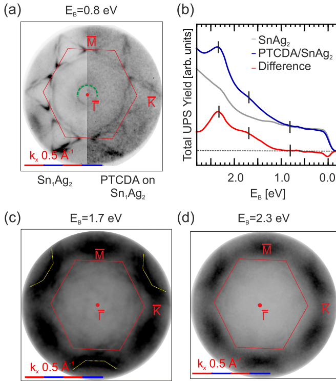
FIG. 5. (a) Constant energy map at 0.8 eV binding energy for the bare \text{SnAg}_2 surface alloy (left) and after adsorption of one layer of PTCDA (right). The hybrid interface state (indicated by a green ring) is not altered upon adsorption of PTCDA. (b) Total UPS yield of the electronic valence structure of PTCDA/ \text{SnAg}_2 (blue), \text{SnAg}_2 (gray), and the difference signal (red). We observe no molecular features at E_F , but two at E_B = 1.7 eV and E_B = 2.3 eV. (c), (d) Symmetrized constant energy maps extracted at E_B = 1.7 eV and E_B = 2.3 eV, respectively, i.e., at the binding energy of the molecular features in the UPS spectrum.
