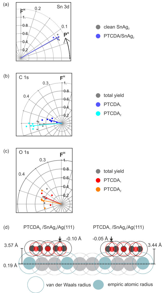
FIG. 4. (a) Argand diagram illustrating the NIXSW results for the Sn species of the \text{SnAg}_2 surface alloy, prior and after the adsorption of a monolayer of PTCDA. (b), (c) Argand diagram for the results of the C 1s and O 1s core levels, respectively, of a PTCDA monolayer on \text{SnAg}_2 . (d) Real-scale vertical adsorption geometry model for PTCDA adsorbed on \text{Sn}_1\text{Ag}_2 surface alloy.
