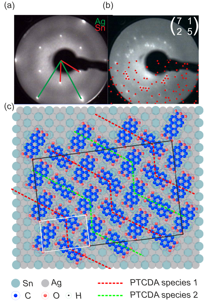
FIG. 1. (a) LEED image recorded for SnAg 2 surface alloy formed on Ag(111) ( E_{\text{kin}} = 76 eV). The unit cell basis vectors of the substrate in momentum space are indicated in green, the one of the (\sqrt{3} \times \sqrt{3})R30^\circ superstructure in red. (b) LEED image for a monolayer of PTCDA on SnAg 2 surface alloy ( E_{\text{kin}} = 14 eV). The bottom half of the LEED image is superimposed with simulated diffraction spots of the superstructure matrix of PTCDA/Ag(111): \begin{pmatrix} 7 & 1 \\ 2 & 5 \end{pmatrix} . (c) structural model of the PTCDA monolayer film on the SnAg 2 . The small unit cell with two PTCDA molecules is marked in white, the larger unit cell that is commensurate with the SnAg 2 superstructure in black.
