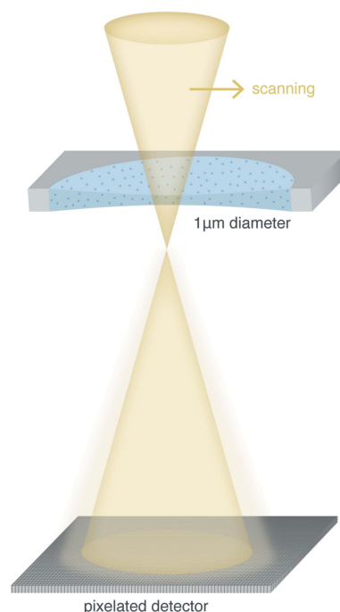
Figure 5 Schematic illustration of cryo-ptychography. A small convergent electron beam scans through the specimen (shown within 1 μm hole) at a certain defocus. A high-speed pixelated detector is used for recording diffractograms that are subsequently collected from partially overlapping sample positions.
