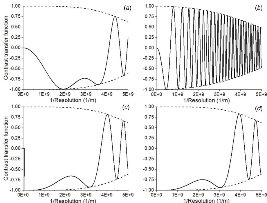
Figure 1 Contrast transfer function of (a) conventional TEM at Scherzer defocus, \Delta f_{\text{Sch}} = 87 nm; (b) conventional TEM at defocus, \Delta f = 1.2 \mu\text{m} ; (c) with phase plate at defocus of 0.6 \Delta f_{\text{Sch}} = 52 nm with cut-on frequency at 1/25 nm ^{-1} ; (d) holography at Gábor defocus, \Delta f_{\text{Gabor}} = 49 nm. All have the illumination semi-angle set at 15 \mu\text{rad} .
