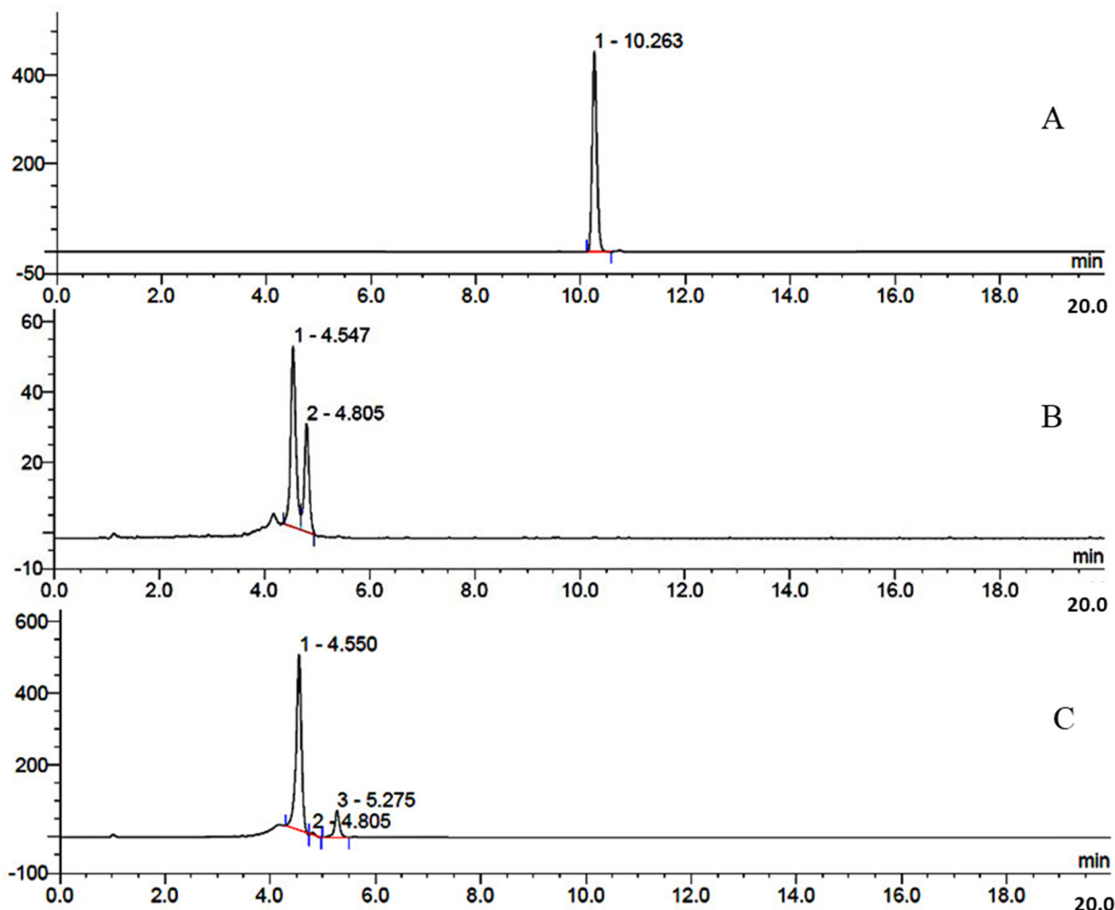
Figure 2. Radio-HPLC analysis of the reaction mixture: (A) radiofluorination of 4 (preparation of 5 ); (B) hydrolysis of 5 with 1.5 N HCl in 50% MeOH; (C) hydrolysis of 5 with 0.5 N HCl in 50% MeOH. HPLC conditions: column: XBridge ® C18 5 \mu\text{m} , 150 \times 4.6 mm (Waters, Millford, CT, USA); gradient: 0–2 min: 2% MeCN (0.1% TFA), 2–13 min: 2–90% MeCN (0.1% TFA); flow rate: 2.0 mL/min; R_t of 5 : 10.3 min; R_t of 6-L- ^{18}\text{F} FMT: 4.6 min.
