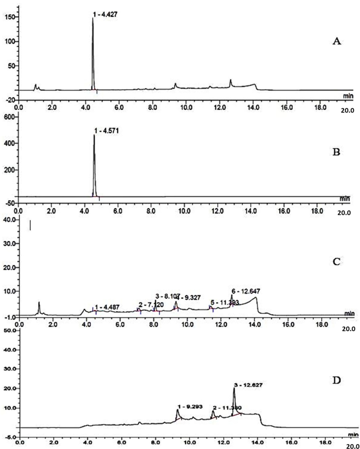
Figure 3. Quality control of 6-L-[ 18 F]FMT: (A) 6-DL-FMT, UV trace ( \lambda = 254 nm); (B) 6-L-[ 18 F]FMT, radioactivity trace; (C) 6-L-[ 18 F]FMT, UV trace ( \lambda = 254 nm); (D) injection of the starting eluent (2% MeCN (0.1% TFA)), UV trace ( \lambda = 254 nm); HPLC conditions: column: XBridge ® C18 5 \mu m, 150 \times 4.6 mm (Waters, Millford, CT, USA); gradient: 0–2 min: 2% MeCN (0.1% TFA), 2–13 min: 2–90% MeCN (0.1% TFA); flow rate: 2.0 mL/min; R_t of 6-L-[ 18 F]FMT: 4.6 min; (D) blank UV chromatogram at 254 nm. Please, notice that the diffuse peak at 3.8–14.0 min and peaks at 3.9; 4.5; 7.2; 8.1; 9.3; 11.4; and 12.6 min (UV 254 nm) are also visible if the starting eluent is injected under the same chromatographic conditions.
