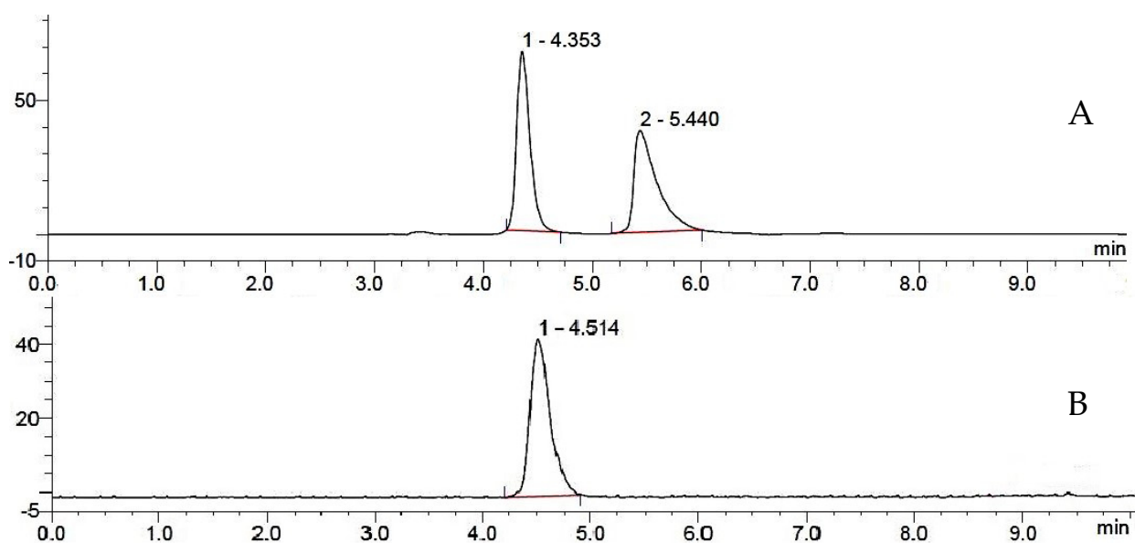
Figure 4. Determination of enantiomeric purity of 6-L-[ ^{18}\text{F} ]FMT by chiral HPLC: (A) 6-DL-FMT, UV trace ( \lambda = 254 nm); peak 1-6-L-FMT; peak 2-6-D-FMT; (B) 6-L-[ ^{18}\text{F} ]FMT, radioactivity trace. HPLC conditions: column Chirobiotic T 150 \times 4.6 mm (Astec, Whippany, NJ, USA); eluent: 10% EtOH in 0.1% Et 3 NOAc; flow rate: 1.0 mL/min.
