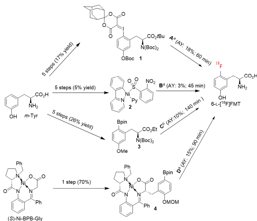
Figure 1. Preparation of 6-L-[ ^{18}\text{F} ]FMT via late-stage radiofluorination with [ ^{18}\text{F} ]fluoride. Radiolabeling conditions: (A) (i) azeotropic drying of [ ^{18}\text{F} ]Et _4\text{NF} /Et _4\text{NHCO}_3 ( \times 3 ), (ii) DMF, 120 ^\circ\text{C} , 20 min [24]; (B) [ ^{18}\text{F} ]KF/K _2\text{CO}_3 /18-crown-6, 1,1'-(phenyl- \lambda^3 -iodanediyl)bis(4-methoxypyridin-1-ium) trifluoromethanesulfonate, MeCN, r.t., 5 min [25]; (C) (i) azeotropic drying of [ ^{18}\text{F} ]KF/K _2\text{C}_2\text{O}_4 /K2.2.2 ( \times 5 ), (ii) Cu(py) _4 (OTf) _2 , DMF, 120 ^\circ\text{C} , 20 min, air [29]; (D) [ ^{18}\text{F} ]Et _4\text{NF} /Et _4\text{NHCO}_3 , Cu(py) _4 (OTf) _2 , n BuOH/DMA, 110 ^\circ\text{C} , 15 min, air [34]. Procedures (B) and (D) avoid any azeotropic drying steps. a —manual synthesis; b —synthesis in a remotely controlled unit. AY—activity yield of the HPLC purified 6-L-[ ^{18}\text{F} ]FMT [13]; r.t.—room temperature.
