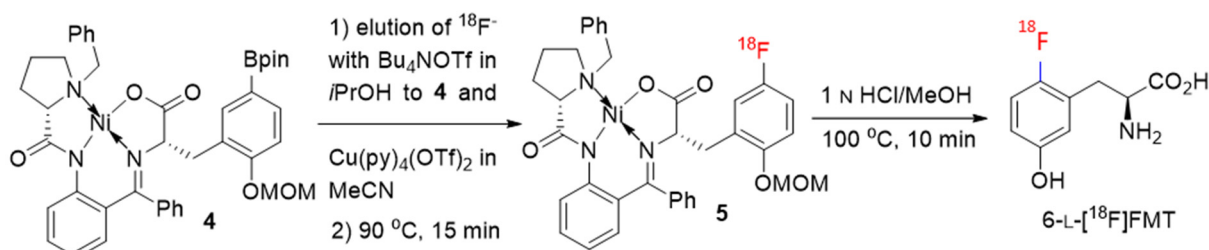
Scheme 1. Radiosynthesis scheme for 6-L-[ 18 F]FMT by Cu-mediated radiofluorination of 4.
