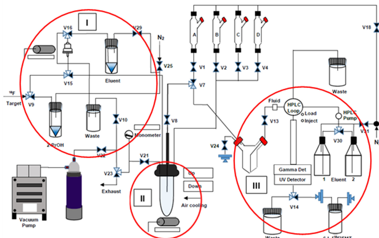
Figure 5. Schematic diagram of the GE TRACERlab FX-C Pro module modified for the preparation of 6-L-[ ^{18}\text{F} ]FMT. A: empty vessel; B: 0.5 N HCl in 50% MeOH (1 mL); C: MeOH (0.5 mL); D: 0.1% AcOH (1.5 mL); RV: 4 (7.7 mg, 10 \mu\text{mol} ) and \text{Cu}(\text{py})_4(\text{OTf})_2 (11 mg, 16 \mu\text{mol} ) in MeCN (0.3 mL); eluent vial: \text{Bu}_4\text{NOTf} (5 mg, 12.5 \mu\text{mol} ) in i PrOH (0.8 mL). RV—reaction vessel (2 mL).
