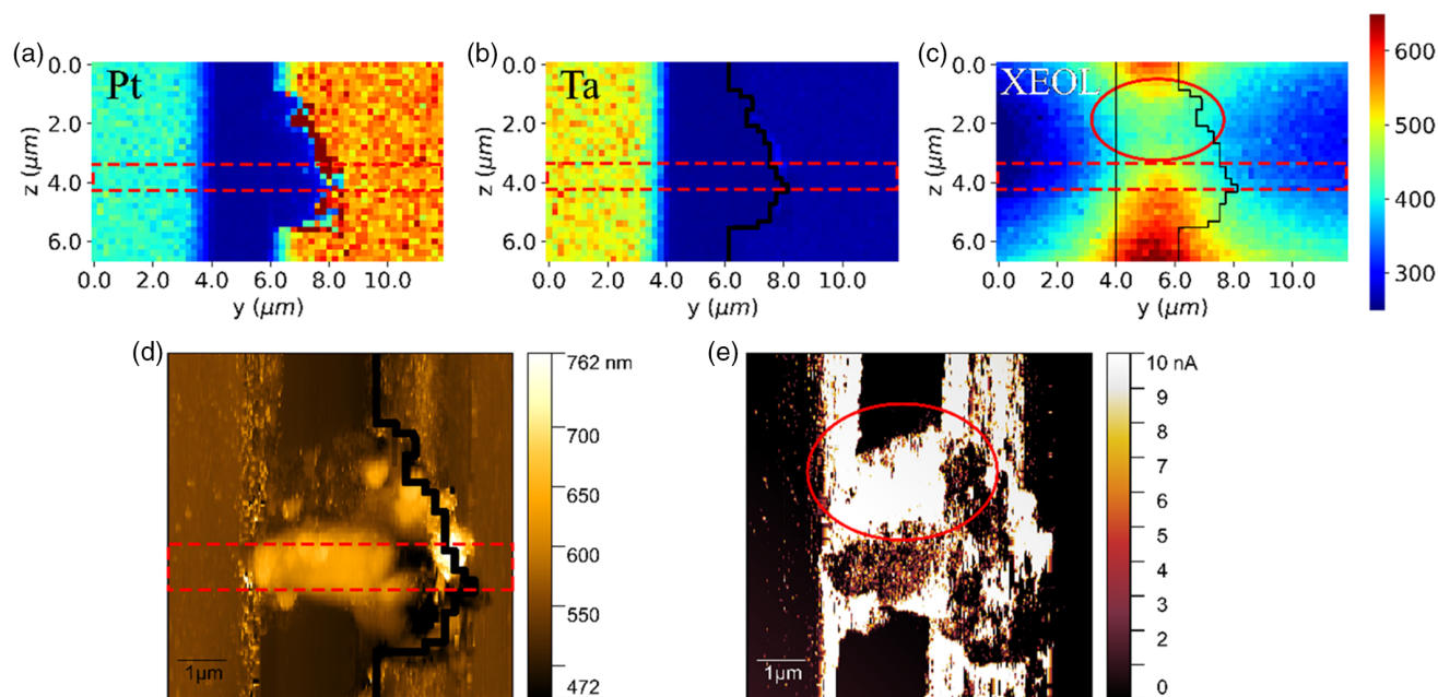
Figure 7. a,b) Typical XRF maps collected for a second-campaign sample (annealed, 1.9 \mu\text{m} gap) after irradiation and electroforming, corresponding to Pt–L (a) and Ta–L (b) lines. c–e) Corresponding XEOL (c), topographic (d), and C-AFM (e) images after irradiation and electroforming are also displayed. The dashed red boxes highlight the irradiated region, and the solid red circles indicate the minimum in the XEOL (c) and the maximum in the C-AFM (e) signals.
