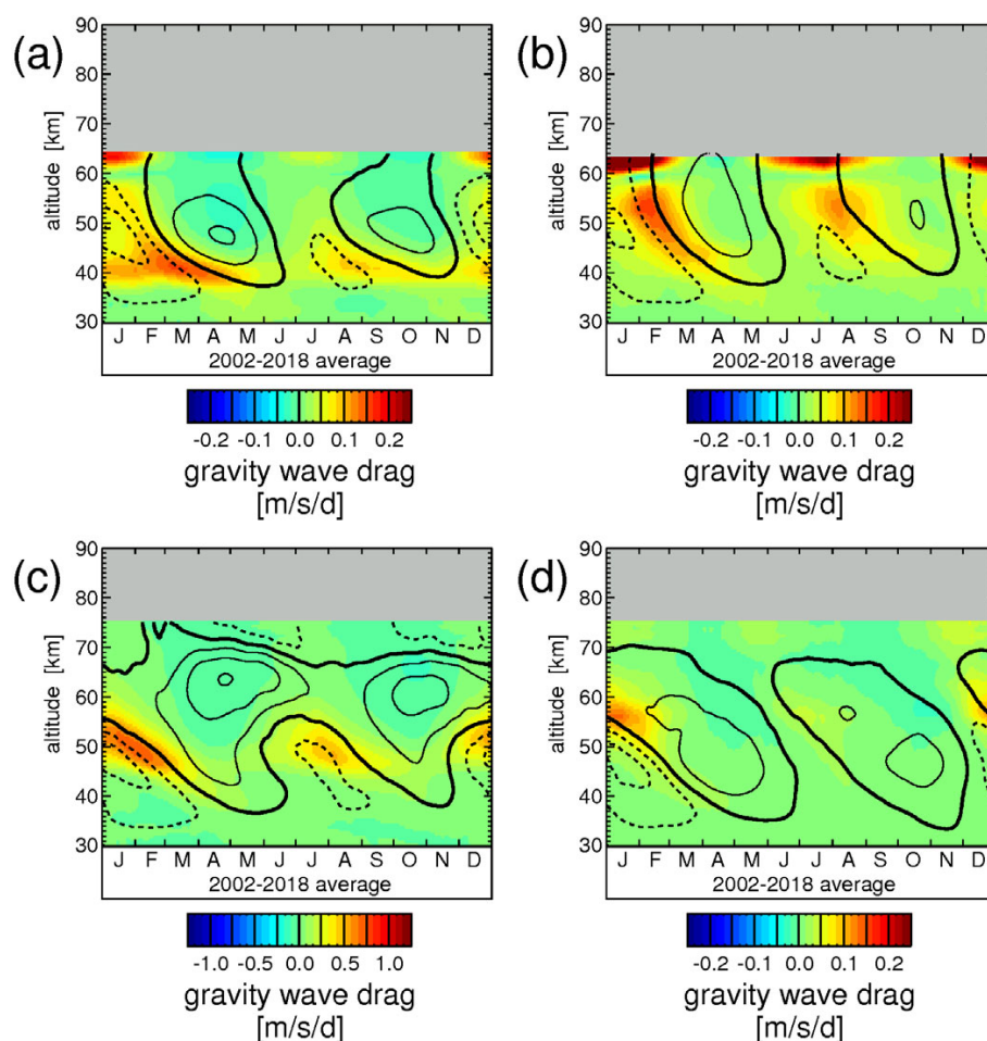
Figure 5. Same as Fig. 4 but for the zonal gravity wave drag \overline{X}_{\text{res}}(k > 20) of model-resolved gravity waves at zonal wavenumbers exceeding k = 20 .
