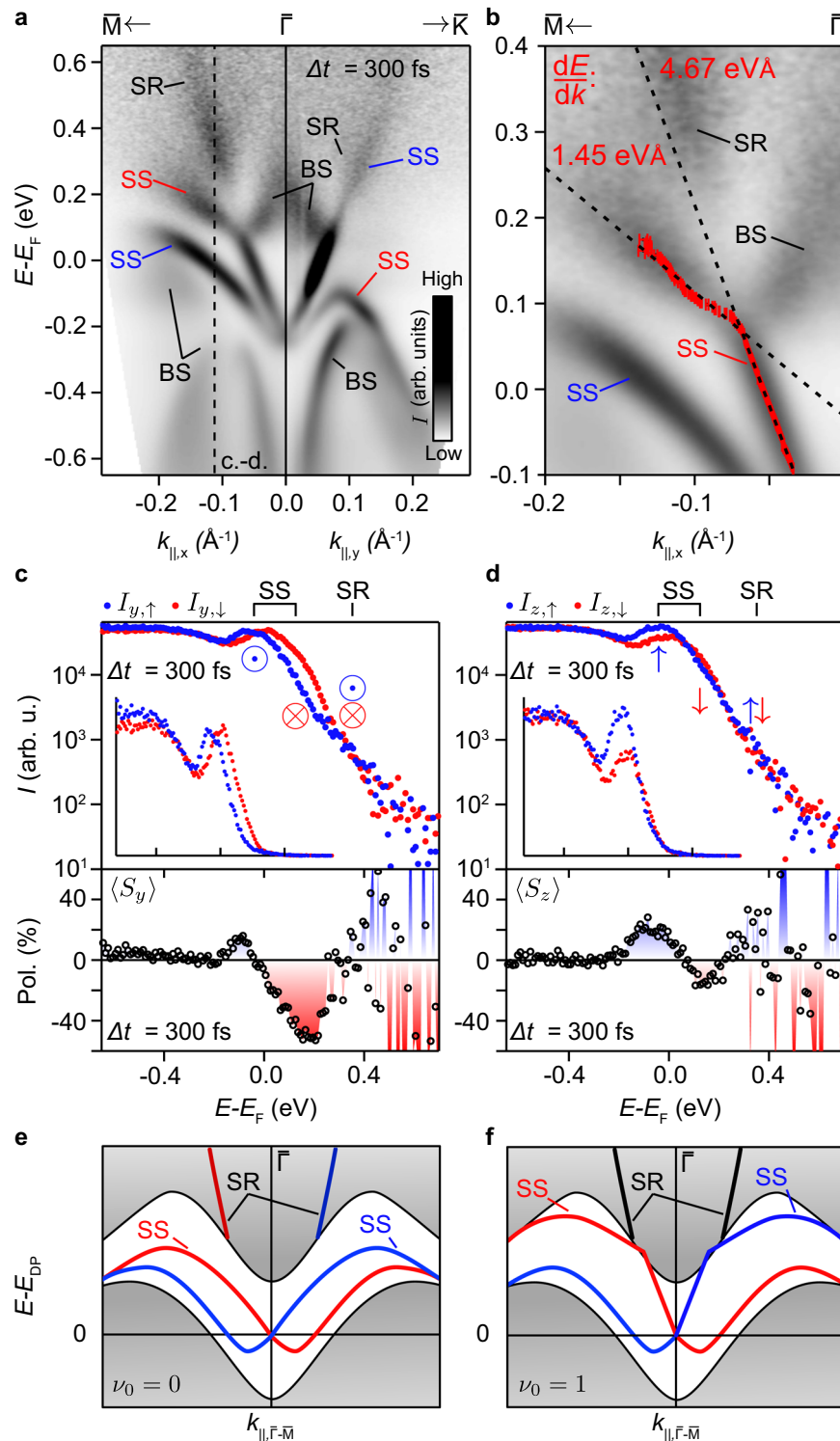
Fig. 2 Experimental characterization of the nonequilibrium band structure. a Energy-momentum dispersion of Sb(111) along the \bar{M}-\bar{\Gamma}-\bar{K} direction measured by time- and angle-resolved photoemission (tr-ARPES) at a time delay \Delta t = 300 fs after optical excitation. Photoemission intensity is given in arbitrary units (arb. u.). Surface-state bands, bulk-derived surface resonances and pure bulk states are denoted as SS, SR, and BS, respectively. To increase the visibility of higher-energy states, the spectra have been normalized by a Fermi function with k_B T \approx 175 meV. b Zoom-in on the region of mass enhancement along the \bar{M}-\bar{\Gamma} direction. Extracted band positions are shown in red. Dashed black lines are linear fits to the band positions either side of the bulk-surface connectivity point, with corresponding group velocities indicated. c, d Spin-resolved tr-ARPES energy distribution curves (blue/red circles for spin up/down respectively) and spin polarizations (pol., black open circles) corresponding to c the in-plane chiral ( S_y ) and d out-of-plane ( S_z ) spin components, taken at the momentum position indicated in a and at a time delay of \Delta t = 300 fs. The spectra are displayed on a logarithmic scale to increase visibility above E_F . The insets reproduce the data on a linear scale. Peaks are labeled according to the corresponding band features. Schematic illustrations which based on the measured band structure depict two possible scenarios where the bulk connectivity of surface states is consistent with (e) a topologically trivial (topological invariant \nu_0 = 0 ) and (f) a topologically nontrivial ( \nu_0 = 1 ) system. Red/blue colors denote opposite spin states.
