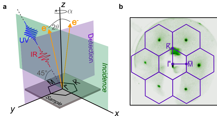
Fig. 1 Experimental geometry and sample characterization. a The infrared (IR) pump (1.5 eV) and ultraviolet (UV) probe (6 eV) fs pulses impinge the sample under an angle of 45°. The electron emission and light incidence planes are orthogonal to each other, and fixed with respect to the laboratory reference frame. The detection plane (spanning over an angle of 2\theta ) was oriented along the \bar{\Gamma} - \bar{K} or \bar{\Gamma} - \bar{M} direction by an azimuthal ( \alpha ) rotation of the sample around the z axis. b Low-energy electron diffraction image (incident electron energy of 98.6 eV) of clean Sb(111), with the surface Brillouin zone shown as solid purple lines.
