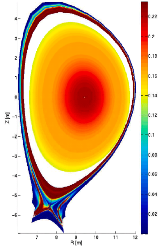
Fig. 2. 2D radiation density map for EU-DEMO flat-top – units are \text{MW/m}^3 . The core values have been calculated with ASTRA, the SOL values are taken from a SOLPS detached case with fluid neutrals. The impact of the non-perfect matching of the two contributions is discussed in the main text.
