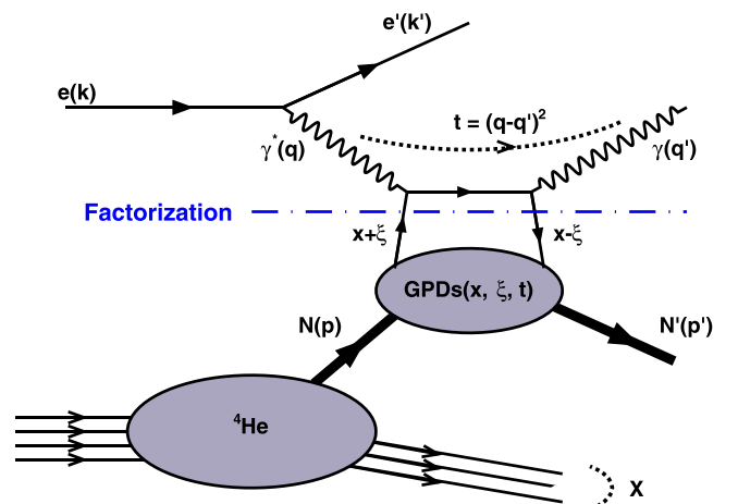
FIG. 5. Diagram representing the incoherent nuclear DVCS.
