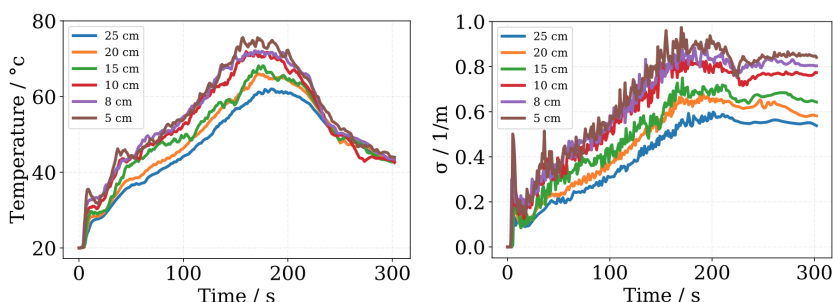
Figure 3: Sensitivity of temperature (left) and extinction coefficient (right) w.r.t. the numerical grid resolution.
