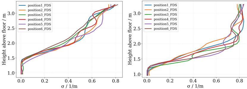
Figure 4: Simulation results at t = 150 s (left) and t = 250 s (right) for the light extinction coefficient profiles at six selected positions in the compartment.
