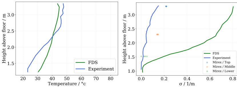
Figure 6: Simulation results for the temperature development (left) and light extinction coefficient (right) at t = 300 s as a function of height.
