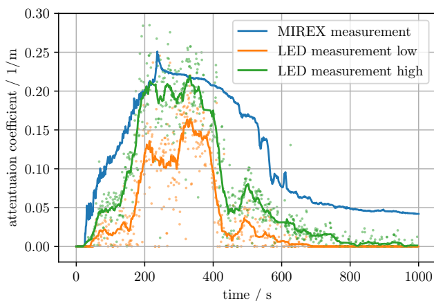
Figure 2: Comparison of a MIREX measurement with the results of the LED-measurements. The data based on the LED measurement shows the results of an optimisation towards low as well as high extinction coefficients.
