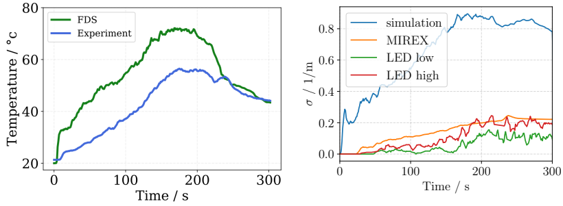
Figure 5: Simulation results for the temperature development (left) and light extinction coefficient (right) during the experiment.
