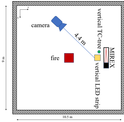
Figure 1: Top view of the experimental setup. [4]
