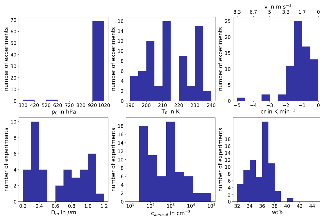
Figure B1. Overview of experimental conditions. The six histograms show the distribution and the parameter range of starting pressure p_0 , starting temperature T_0 , cooling rate cr , vertical velocity v , median aerosol particle diameter D_m , aerosol particle number concentration c_{\text{aerosol}} and weight percentage wt % of H 2 SO 4 in the aqueous solution particles before experiment start.
