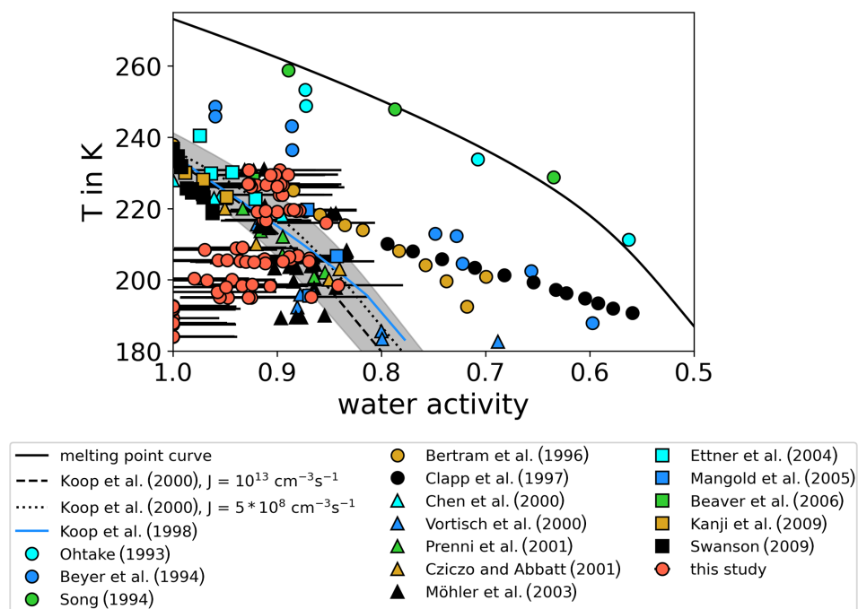
Figure C1. Summary of homogeneous freezing measurements of \text{H}_2\text{SO}_4/\text{H}_2\text{O} solutions in the a_w – T space. The homogeneous freezing onsets of sulfuric acid solution samples shown in Fig. 1 are complemented by the AIDA results from this study (red points). The results in the S_{\text{ice}} – T space were converted into the a_w – T space by assuming equilibrium conditions a_w = \text{RH}_w and by using the parameterizations for the water vapor saturation pressures with respect to ice and supercooled liquid water given by Murphy and Koop (2005). The uncertainties of the calculated a_w values vary between \pm 0.036 and \pm 0.076 .
