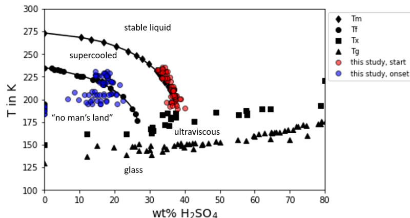
Figure D1. Phase diagram of sulfuric acid adapted from Koop (2004). The phase diagram of sulfuric acid as given by Koop (2004) and references therein is shown and complemented by the calculated weight percentage concentrations of the sulfuric acid aerosol particles before the start of the AIDA experiments of this study (red dots) and at the observed ice onset during the experiments (blue dots).
