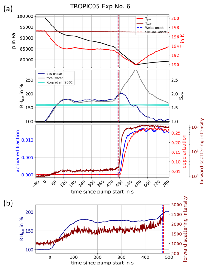
Figure 5. Investigation of kinetic limitations with respect to water uptake in the AIDA chamber. (a) This panel is composed in the same way as Fig. 3. For the experiment shown, started at about 197 K, the pump rate was controlled in such a way that the relative humidity with respect to ice stayed relatively constant for about 5 min at about 170 % and hence above the homogeneous freezing threshold suggested by Koop et al. (2000). For details on this experiment, see Sect. 3. (b) Enlarged view of the relative humidity and the forward scattering intensity at the beginning of the experiment.
