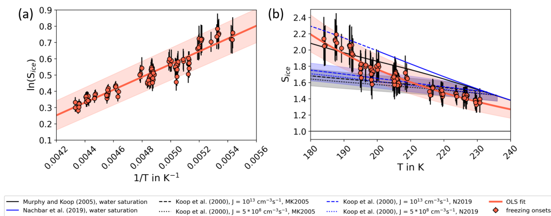
Figure 6. New fit line for homogeneous freezing onsets of \text{H}_2\text{SO}_4/\text{H}_2\text{O} aerosol particles. (a) The freezing onsets determined by OPC and SIMONE data (red dots) are shown in an Arrhenius plot and fitted by an ordinary least square (OLS) fit with the form \ln(S_{ice}) = a + \frac{1}{T} \cdot b . The parameters are a = -1.40 \pm 0.05 and b = 390 \pm 10 \text{ K} , and the goodness of the fit is R^2 = 0.92 . The shaded area indicates the uncertainty of the fit parameters. (b) The OLS fit shown in panel (a) is transferred into the S_{ice} – T space and compared to Koop2000 and the water saturation lines suggested by Murphy and Koop (2005) and Nachbar et al. (2019). The blue and grey shaded areas indicate the uncertainties of Koop2000 ( \pm 5\% in water activity) as given in Koop (2004).
