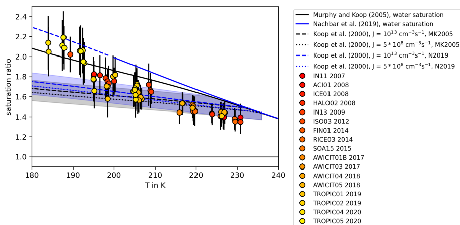
Figure 4. Homogeneous freezing onsets of \text{H}_2\text{SO}_4/\text{H}_2\text{O} aerosol particles. The freezing onset conditions, T_{\text{ice}} and S_{\text{ice,fr}} , are displayed in comparison with the homogeneous freezing thresholds suggested by the WAC-based predictions by Koop et al. (2000) (dashed and dotted lines) using two different parameterizations for the water saturation pressure with respect to supercooled liquid water from Murphy and Koop (2005) (MK2005, black) and Nachbar et al. (2019) (N2019, blue). The blue and grey shaded areas indicate the uncertainties of the WAC-based predictions ( \pm 5\% in water activity) as given in Koop (2004). The used water saturation pressures with respect to supercooled liquid water according to MK2005 (solid black line) and N2019 (solid blue line) are also shown. The colors of the measurement data points represent the different AIDA campaigns in the corresponding years. The oldest campaigns are presented in reddish colors, whereas the more recent campaigns are shown in yellowish colors.
