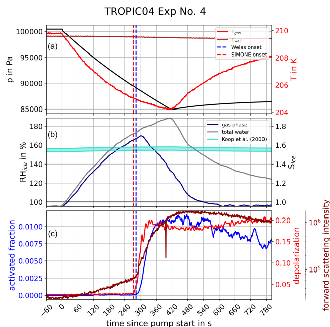
Figure 3. Time series of a typical AIDA homogeneous freezing experiment. The upper panel shows the course of pressure (black), as well as gas (red) and wall (dark red) temperatures, inside the AIDA chamber as a function of time since pump start at t = 0 . Accordingly, the middle panel shows the course of relative humidity with respect to ice \text{RH}_{\text{ice}} and ice saturation ratio S_{\text{ice}} of gas-phase (blue) and total water (grey). The turquoise area marks the range of freezing onset saturation ratios according to Koop et al. (2000). In the lower panel, the activated fraction of \text{H}_2\text{SO}_4/\text{H}_2\text{O} particles determined by OPC data (blue) and the forward scattering intensity (dark red) as well as the backscattering depolarization ratio (red) derived from SIMONE light scattering measurements are presented. The time of homogeneous freezing onsets derived from the activated fraction (blue) and from the SIMONE measurements (red) are marked by the vertical dashed lines.
