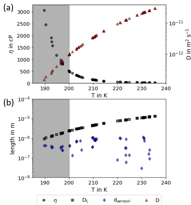
Figure D2. Viscosity and diffusion coefficients for the start conditions of the AIDA experiments. (a) Viscosity (black dots) and diffusion coefficients (red triangles) calculated using the parameterization of Williams and Long (1995) and the Stokes–Einstein equation. (b) Comparison of the mean particle diameter of the sulfuric acid particle population (blue diamonds) to the diffusion length of water molecules (black squares) on a timescale of 6 s. Note that the shown data points represent the starting conditions of the AIDA experiments. As the parameterization of Williams and Long (1995) is only valid for T > 200 K, the data points of experiments at lower temperatures are displayed in a grey shaded box.
