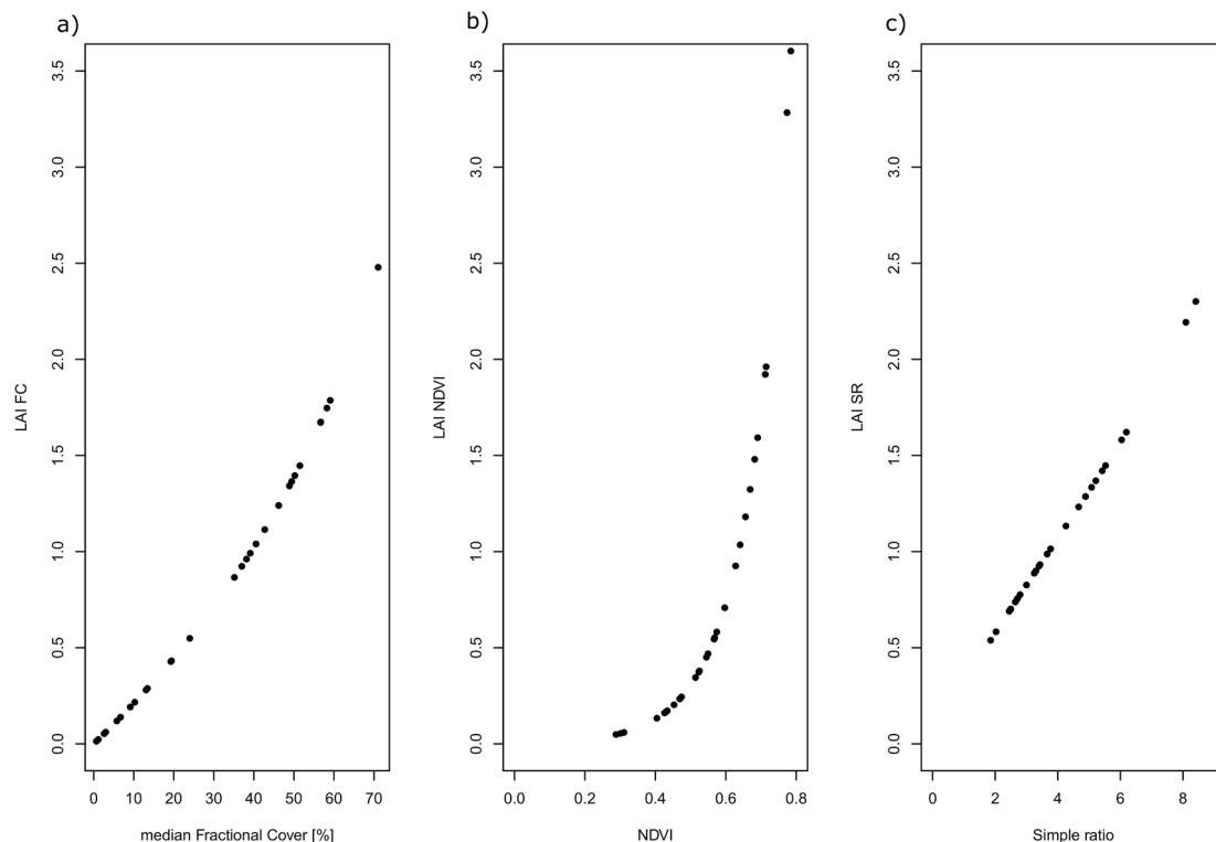
Fig. 6. Retrieved understory LAI in relation to its main parameter - fractional cover [%], NDVI, and SR, respectively. Black dots represent the mean LAI u of the investigated sites.
