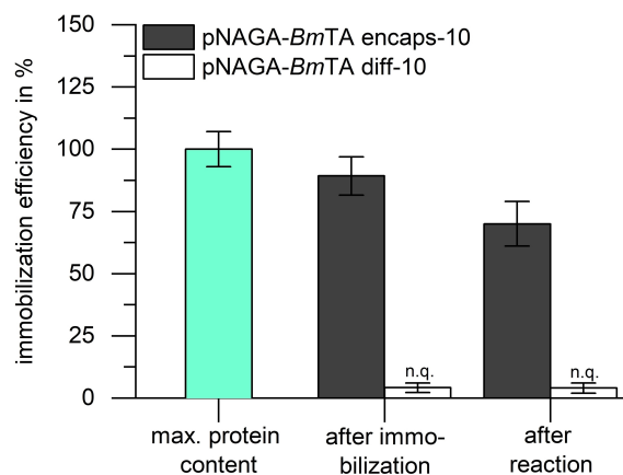
Figure 2. Immobilization efficiency (%) of BmTA in poly( N -acryloyl glycineamide) (pNAGA) hydrogels that were loaded by encapsulation (encaps-X) or diffusion (diff-X). The X represents the amount of BmTA applied for loading which was 10 µg protein per mg gel dry weight. Immobilization was determined using an adapted Bradford assay for dissolved hydrogels ( n = 3).
