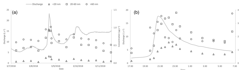
FIGURE 4 Variation of P concentration within the three fractions during the (a) March and (b) May event
