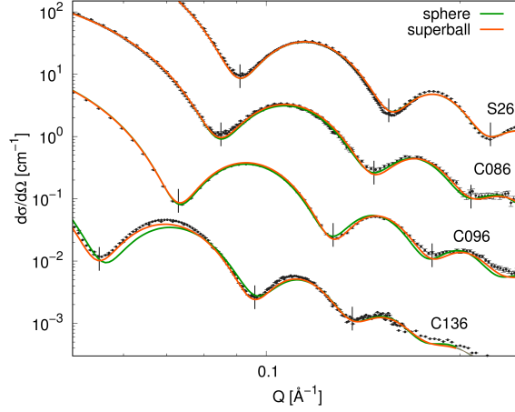
Figure 3: Small-Angle X-ray Scattering (SAXS) by iron oxide nanospheres and nanocubes, refined using a sphere and superball form factor. Detail of Fig. 2b. The first three form factor minima in the experimental data are indicated with a vertical marker.
