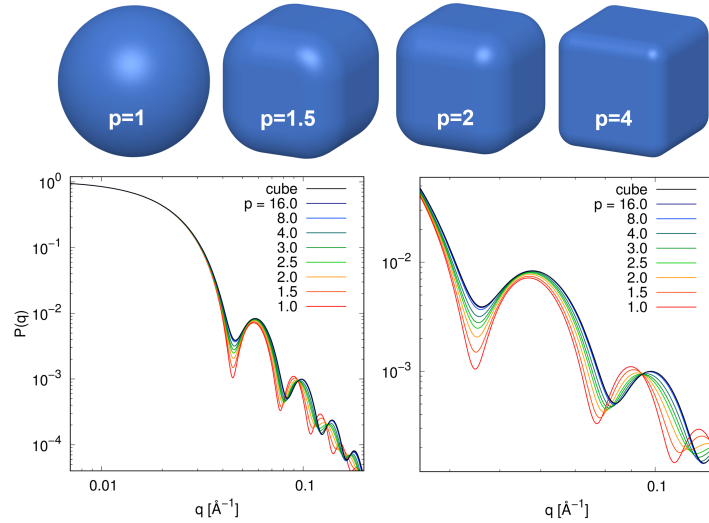
Figure 1: Visualization of the superball shape for selected shape parameters p (top) and its corresponding form factor in comparison to a cube form factor simulated for a particle size distribution of \sigma_r = 5\% (bottom left), with a magnification of the first three form factor minima (bottom right).
