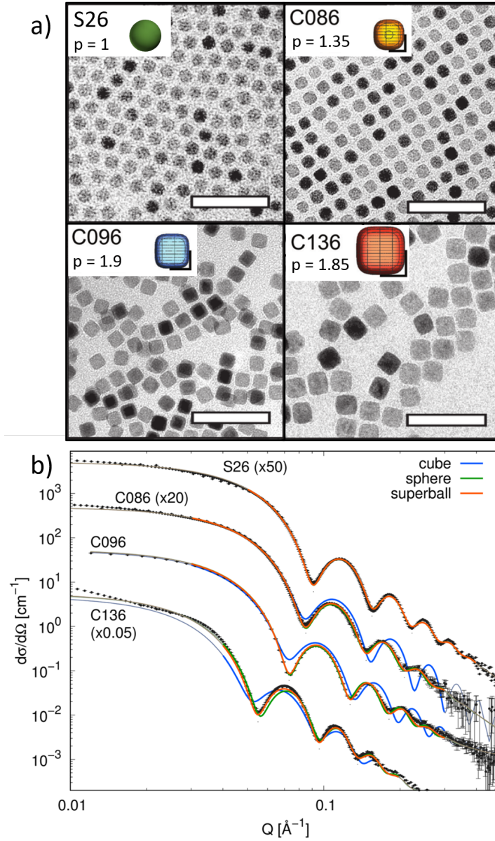
Figure 2: a) Transmission Electron Microscopy (TEM) images of iron oxide nanoparticles with varying shape parameter p as determined from HRTEM. Scale bars: 50 nm. Adapted from Wetterskog et al. 26 and Wetterskog et al. 44 b) Experimental Small-Angle X-ray Scattering (SAXS) by iron oxide nanospheres and nanocubes (symbols). Refinements using a cube, sphere, and superball form factor are shown. Color of the fit indicates the q range used for fitting, whereas grey lines indicate the form factors outside the fit ranges. Data scaled for clarity as indicated.
