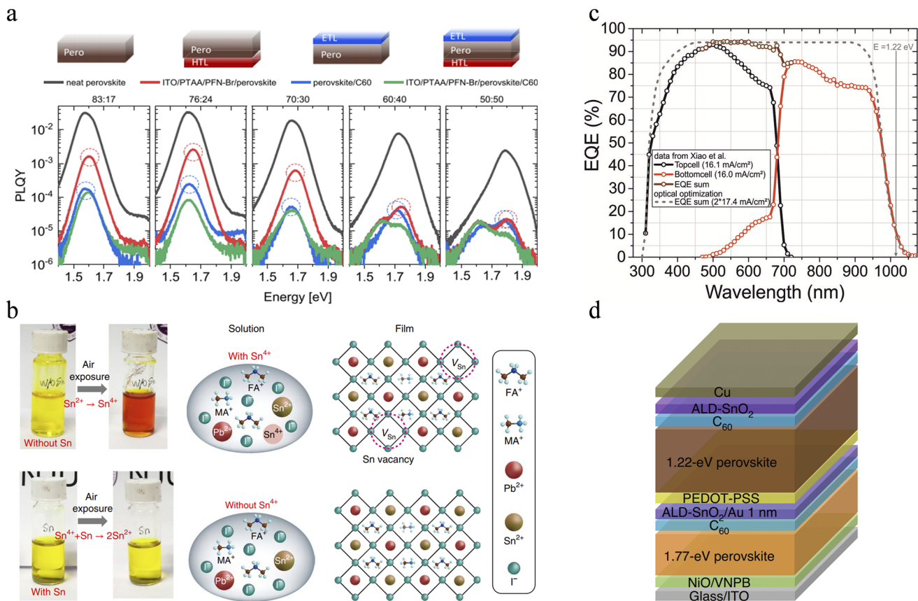
FIG. 27. (a) Photoluminescence quantum yield (PLQY) spectra of five perovskite compositions of \text{Cs}_{0.05}(\text{FA}_x\text{MA}_{1-x})_{0.95}\text{Pb}(\text{I}_x\text{Br}_{1-x})_3 as indicated by the molar FAI to MABr ratio from 83:17–50:50. Different colors indicate different layer stacks from pure perovskite films (black) to both full as indicated. Reprinted with permission from Peña-Camargo et al. , ACS Energy Lett. 5 , 2728 (2020). Copyright 2020 American Chemical Society. (b) Photographs exhibit the oxidation of \text{Sn}^{2+} to \text{Sn}^{4+} in ambient air and reduction of \text{Sn}^{4+} to \text{Sn}^{2+} with metallic Sn powder. Meanwhile, the illustration of the Sn vacancy formation due to the present of \text{Sn}^{4+} and the suppression of Sn vacancies with metallic Sn powder in the Sn–Pb perovskite precursor and film. Reprinted with permission from Lin et al. , Nat. Energy 4 , 864 (2019). Copyright 2019 Nature Publishing Group. (c) EQE spectra of the best reported all-perovskite tandem solar cell with the EQE of the individual subcells, and the sum value is extracted from Ref. 442. The dashed line refers to an empirical optimization that would allow for the matched photocurrent of 17.4 mA/cm 2 . (d) A schematic architecture of all-perovskite tandem solar cells. Reprinted with permission from Xiao et al. , Nat. Energy 5 , 870 (2020). Copyright 2020 Nature Publishing Group.
