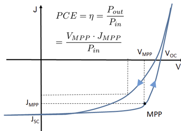
FIG. 32. Possible J–V characteristic (with characteristic values indicated) by perovskite solar cells demonstrating hysteretic behavior as forward and reverse scan directions (indicated by the arrows) leading to different values for the MPP.
