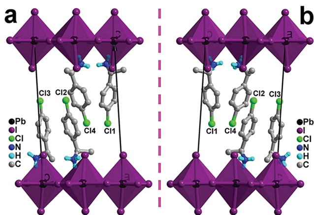
FIG. 9. Crystal structures of (a) [R-1-(4-chlorophenyl)ethylammonium] _2 PbI _4 (R-LIPF) and (b) [S-1-(4-chlorophenyl)ethylammonium] _2 PbI _4 (S-LIPF) 2D lead iodide perovskites, showing a mirror-image relationship. Reprinted with permission from Yang et al. , Adv. Mater. 31 , 1808088 (2019). Copyright 2019 John Wiley and Sons.
