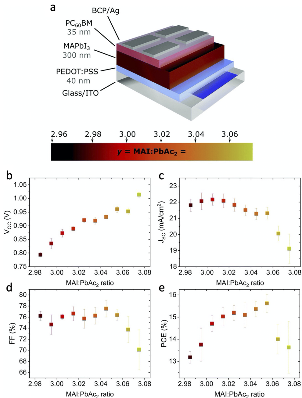
FIG. 34. (a) Schematic of the photovoltaic device architecture: ITO/PEDOT:PSS/MAPbI 3 /PC 60 BM/BCP/Ag and the fitting color scale used throughout the manuscript for illustrating stoichiometric changes of the precursor solution, with the stoichiometry y representing the molar ratio of MAI to PbAc 2 . (b)–(e) Variation of the photovoltaic parameters ( V_{oc} , J_{sc} , FF, and PCE) of solar cells with changing stoichiometry ( 2.985 < y < 3.075 ). Adapted with permission from Fassel et al. , Energy Environ. Sci. 11 , 3380 (2018). Copyright 2018 The Royal Society of Chemistry.
