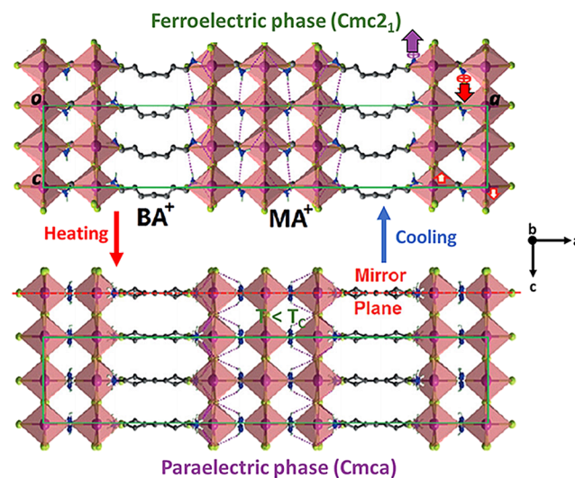
FIG. 10. Ferroelectric (Cmc _2 1) and paraelectric (Cmca) phases of (\text{BA})_2(\text{MA})_2\text{Pb}_3\text{Br}_{10} at 293 and 340 K, respectively. There is a deviation of negative and positive charge centers in the ferroelectric phase compared with the paraelectric phase, which is indicated by the purple and red arrows. Reprinted from Hou et al. , J. Appl. Phys. 128 , 060906 (2020) with the permission of AIP Publishing.
