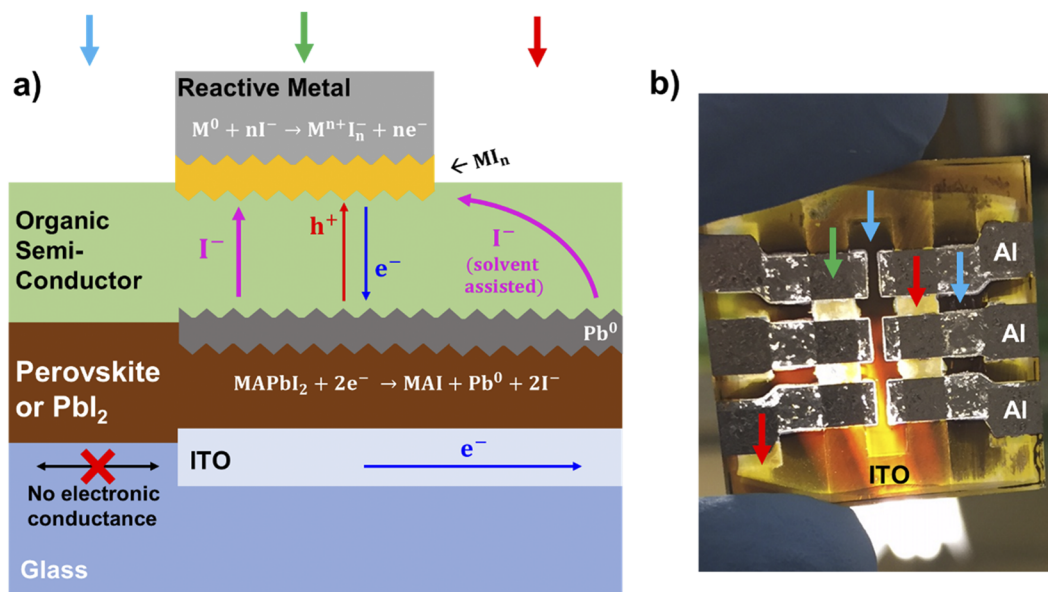
FIG. 39. (a) Mechanism of electrochemical corrosion showing how electrical conduction can facilitate redox over very long distances. (b) Photograph of a device with Al contacts degraded in the dark in atmosphere. The substrate dimensions are 1 \times 1 \text{ in.}^2 , and pixel areas are \sim 0.12 \text{ cm}^2 . The colored arrows point to the indicated regions in (a), highlighting perovskite reacting with the ITO (red arrow) despite being macroscopic distances from the Al, as well as the opposite behavior for glass regions that are electronically isolated from the Al.
