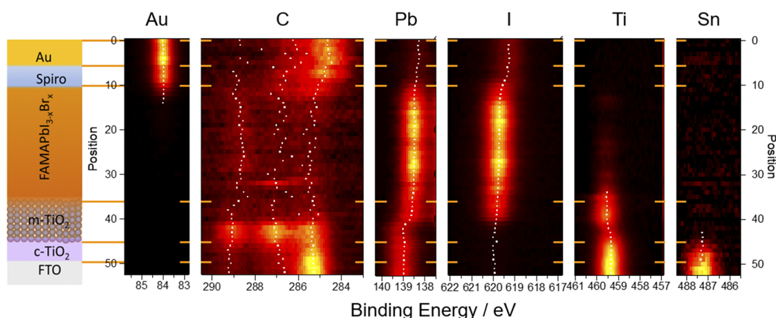
FIG. 23. Intensity contour maps of the XPS line scans performed on the TCS. The following core level spectra are depicted: \text{Au}4f_{7/2} , \text{C}1s , \text{Pb}4f_{7/2} , \text{I}3d_{5/2} , \text{Ti}2p_{3/2} , and \text{Sn}3d_{5/2} . On each scan, the white points correspond to local intensity maxima. The elemental distribution over this TCS leads to the expected PSC architecture sketched on the left. Adapted from Ref. 424.
