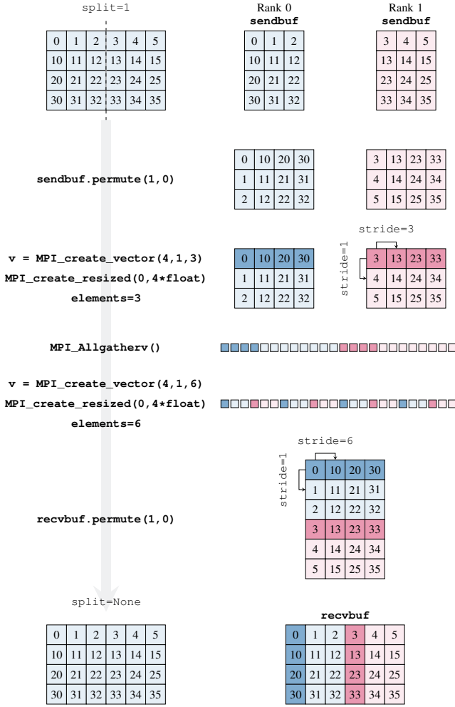
Fig. 3: Internal handling of a resplit(None) operation on a two-dimensional DNDarray with split=1 in HeAT, i.e., data replication on all nodes. It depicts the on-the-fly creation of MPI datatypes for the strided access into the output and input buffers.
