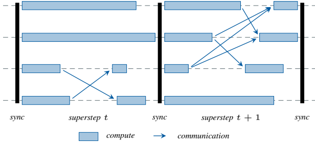
Fig. 1: The BSP-inspired parallel processing model utilized by HeAT. Computation steps are marked as light blue blocks, possible communication as blue arrows, implicit or explicit synchronization points as black vertical bars.
