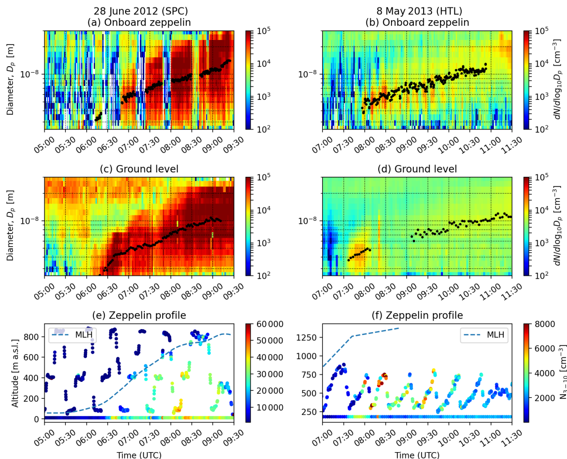
Figure 6. Time evolution of particle number size distributions measured by the NAIS (positive polarity) on board the Zeppelin ( a, b ) and at the ground level ( c, d ) in HTL and in SPC on the 2 case study days. The black dots are the mean mode diameters found by fitting a log-normal distribution over the growing mode. The panels ( e ) and ( f ) show the 3–10 nm particle number concentration as a function of time and altitude on board the Zeppelin and at the ground-based station. The ML height during the measurement flights is also shown.
