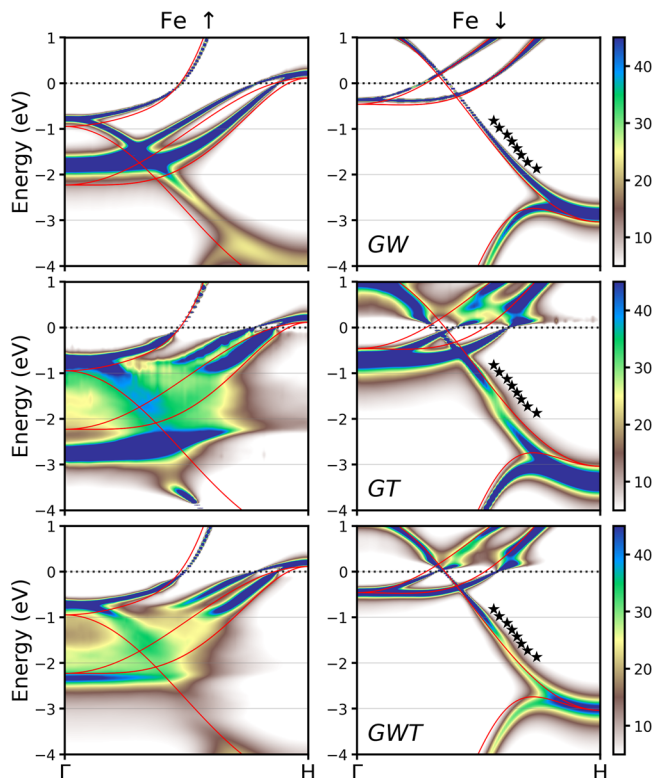
Fig. 4 Renormalized band structures of bcc Fe for \Gamma -H. Majority and minority band structures of bcc Fe renormalized with GW, GT, and GWT self-energies along \Gamma -H. Quasiparticle energies extracted from the ARPES spin-down spectrum in the vicinity of the electron-magnon kink 7 are shown by black stars.
