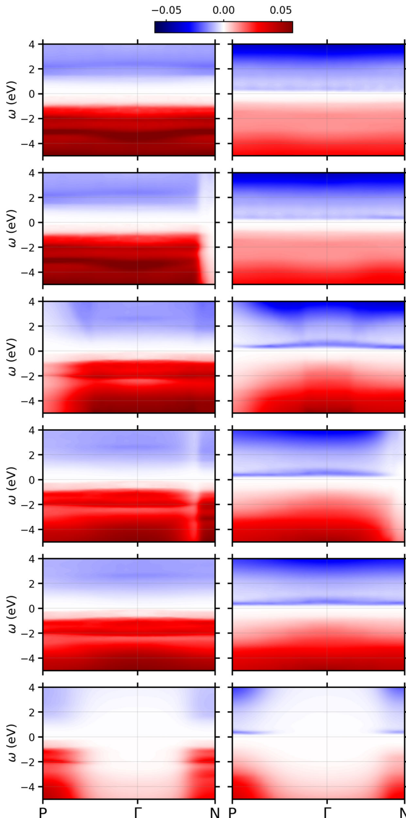
Fig. 6 Momentum and energy dependence of the correlation self-energy in Fe. \text{Im} \Sigma_{kn}^{\sigma}(\omega - \Delta_v) is shown for the lowest bands and both spins (cf. Fig. 1). The bands are ordered with respect to their energy at \Gamma from bottom to top (same order as in Fig. 10 of ref. 19 ).
