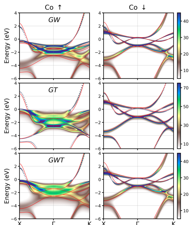
Fig. 7 Renormalized band structures of fcc Co. Spin-dependent band structures of renormalized with GW , GT , and GWT self-energies along X - \Gamma - K .
