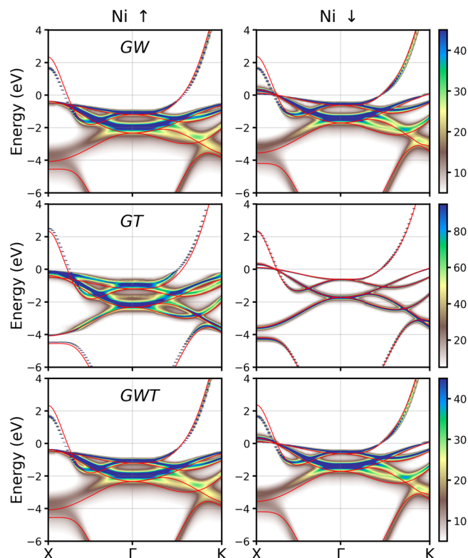
Fig. 8 Renormalized band structures of fcc Ni. Spin-dependent band structures are renormalized with GW , GT , and GWT self-energies along X - \Gamma - K .
