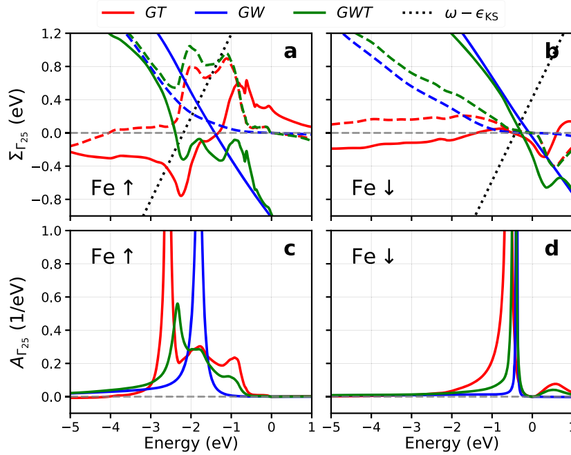
Fig. 5 Self-energies and spectral functions for selected valence states in bcc Fe. The GW, GT, and GWT spin-up and spin-down self-energies (a, b) and spectral functions (c, d) for the triple-degenerate \Gamma_{25} Fe valence states. Solid and dashed lines represent the real and imaginary parts of \langle \varphi_{\mathbf{k}n}^o | \Sigma^o(\omega - \Delta_v) - v_{xc}^o | \varphi_{\mathbf{k}n}^o \rangle (GW and GWT) and \langle \varphi_{\mathbf{k}n}^o | \Sigma^o(\omega - \Delta_v) | \varphi_{\mathbf{k}n}^o \rangle \mp \Delta_x/2 (GT), respectively. The intersections of the real part with the linear function \omega - \epsilon_{\mathbf{k}n}^o are (approximately) the quasiparticle peak positions. The Fermi energy is set at \omega = 0 .
