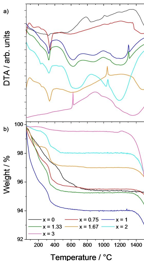
Figure 4. Thermal investigation of the series \text{Na}_3\text{Zr}_{3-x}\text{Si}_2\text{P}_{1.5+x/2}\text{O}_{11.5+x/2} : a) DTA results, and b) TG results.
