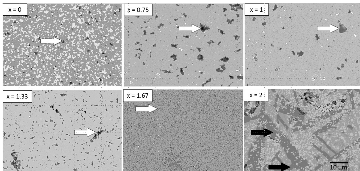
Figure 9. SEM images of polished cross-sections of sintered \text{Na}_3\text{Zr}_{3-x}\text{Si}_2\text{P}_{0.5+x/2} ceramics. The sintering temperatures are listed in Table 1. In the top row, the white phase is \text{ZrO}_2 . The black arrows show the \text{SiO}_2 phase and the white arrows indicate pores.
