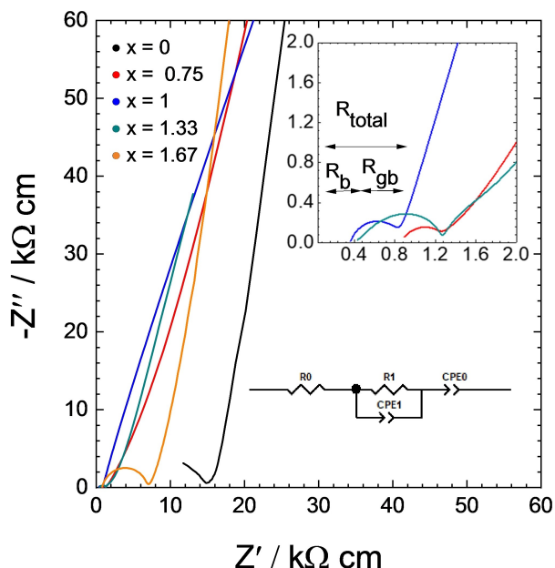
Figure 10. Nyquist plot of impedance spectra at 25 °C of \text{Na}_3\text{Zr}_{3-x}\text{Si}_2\text{P}_x\text{O}_{11.5+x/2} with 0 \leq x \leq 1.67 after accounting for the sample dimensions. The inset shows the magnification of the high frequency region. The resistance contributions in the inset refer to the blue line. The equivalent circuit is also shown.
