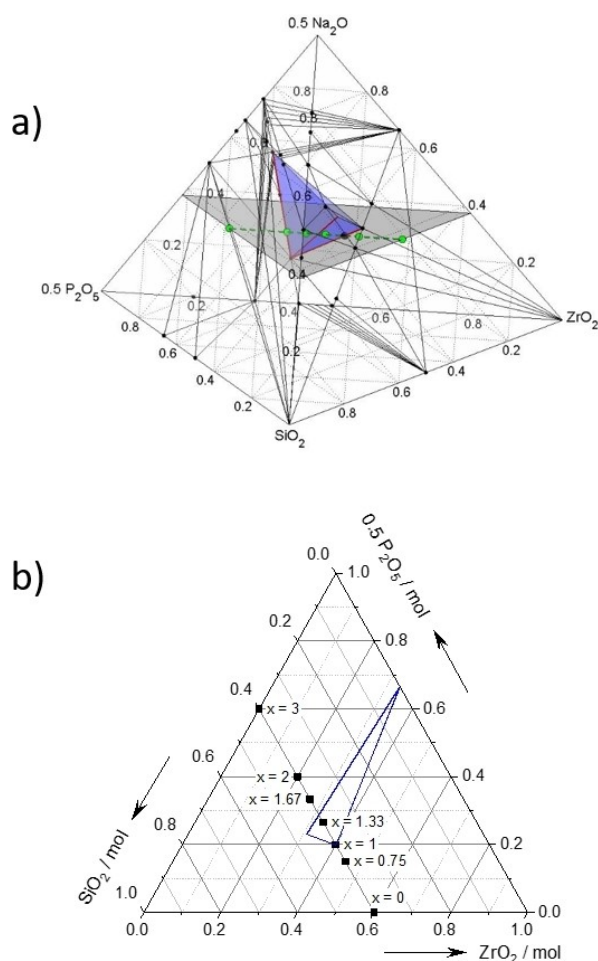
Figure 1. a) The quaternary phase diagram Na_2O-SiO_2-ZrO_2-P_2O_5 visualizing the position of the nominal series Na_3Zr_{3-x}Si_2P_xO_{11.5+x/2} with x = 0, 0.75, 1, 1.33, 1.67, 2 and 3 (from right to left) shown as green circles ( Na_3Zr_2Si_2PO_{12} in dark green). The grey plane indicates compounds with a constant molar fraction of \xi_{Na} = 0.375 . The blue compressed tetrahedron corresponds to the phase field of NaSiCON materials (see [12] for further details). b) Ternary plot of the grey plane in Figure 1a. The blue lines indicate the cross section of the NaSiCON tetrahedron at \xi_{Na} = 0.375 . According to this graph, only the series members with x = 1 and x = 1.33 can be ascribed to the phase field of NaSiCON.
