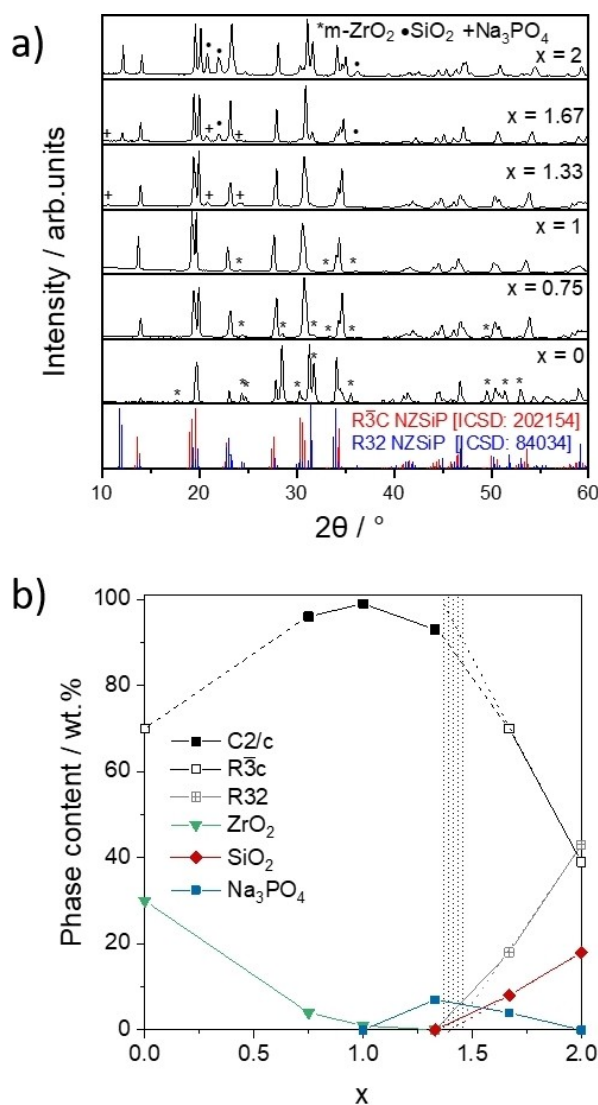
Figure 6. a) XRD patterns of \text{Na}_3\text{Zr}_{3-x}\text{Si}_2\text{P}_2\text{O}_{11.5+x/2} with 0 \leq x \leq 2 after sintering at 1370 °C ( x=0 ), 1250 °C ( x=0.75 ), 1240 °C ( x=1 ), 1230 °C ( x=1.33 ), 1160 °C ( x=1.67 ), 1060 °C ( x=2 ). b) Phase contents determined by Rietveld refinement. Combining the data points in a linear manner at high x values towards 0 and 100% (dotted lines) leads to a common end at x=1.4 – 1.5 , indicating the limit of the C2/c phase region and marked with the vertical dotted region.
