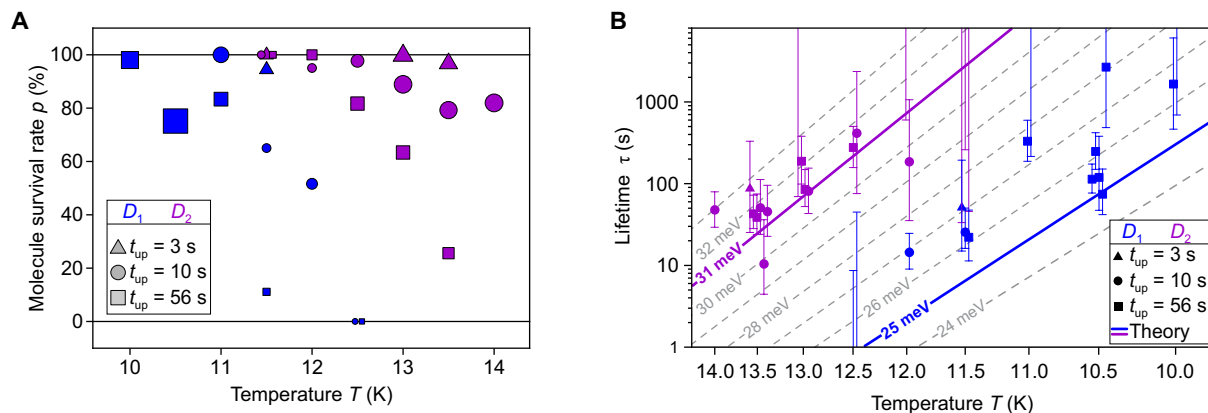
Fig. 4. Temperature-dependent stability of s-PTCDA. (A) Survival rate p = s/n of s-PTCDA molecules on D_1 (blue) and D_2 (purple) pedestals as a function of sample temperature T and duration of tip retraction t_{up} . The symbol size (area) is proportional to the number of trials n on which the respective data point is based (min = 10, max = 200). Higher survival rates facilitate more trials because PTCDA has to be re-erected less frequently. (B) Arrhenius plot of the temperature-dependent lifetimes \tau of D_1 - and D_2 -type s-PTCDA obtained with Eq. 1 for each individual set of experiments. Sets of trials in which the molecule either always or never dropped yield apparent lifetimes of \tau = 0 or \tau = \infty such that the corresponding data points are outside the plot. The uncertainty in \tau is quantified by the 95% Wilson confidence intervals or by the rule of three (31) in cases where t = 0 or t = \infty (see Materials and Methods). Data points at the same temperature are laterally offset for better visibility. The gray isolines represent \tau(T) relations for a set of barrier heights 24 \text{ meV} \leq E_A \leq 33 \text{ meV} (Eq. 2) including the barrier heights obtained by DFT for D_1 (blue) and D_2 (purple). For the isolines, the attempt frequency \omega_0(T) = 2.06 \cdot 10^9 \text{ s}^{-1} \text{ K}^{-1/2} \cdot T^{1/2} was used.
