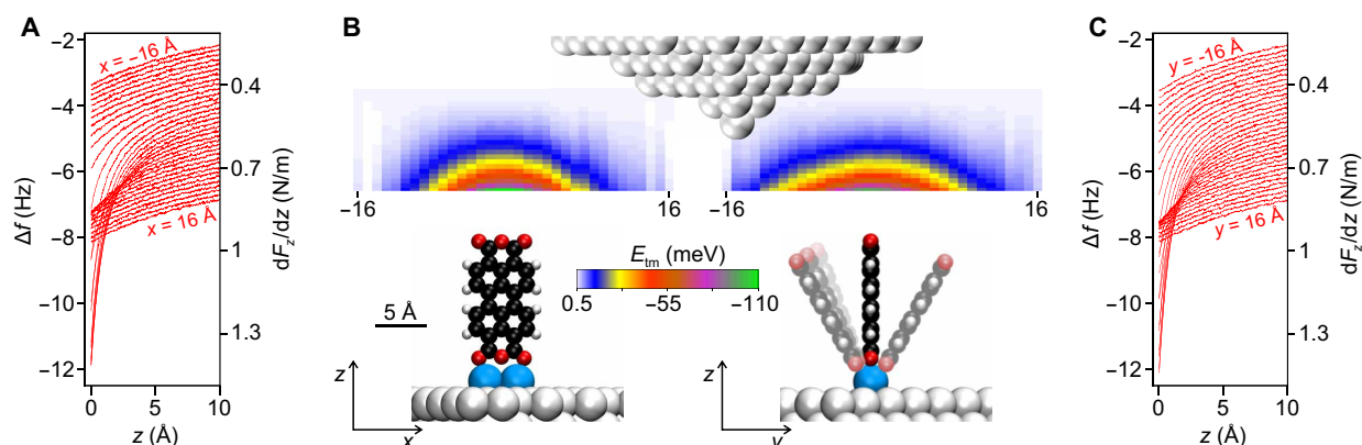
Fig. 2. Tip-molecule interaction potential. (A) The 34 \Delta f(z) curves measured at positions ( -16 \text{ Å} < x < 16 \text{ Å} , y = 0 ) along a line centered above s-PTCDA at ( x = 0 , y = 0 ) and oriented along the PTCDA plane. Each curve is averaged over 10 individual spectra and offset vertically for better visibility ( 0.14 Hz between consecutive curves). (B) Sections of the tip-molecule interaction energy E_{tm}(x, y, z) along the molecular plane (left) and perpendicular to it (right) as obtained from the data in (A) and (C). Maps and s-PTCDA models are drawn and located to scale. (C) The 34 \Delta f(z) curves similar to (A) but measured at positions ( x = 0 , -16 \text{ Å} < y < 16 \text{ Å} ) on a line oriented perpendicular to the PTCDA plane.
