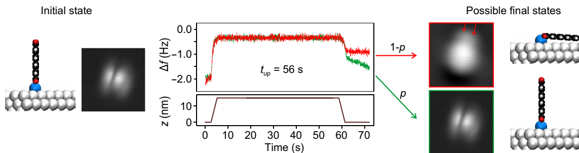
Fig. 3. Measurement protocol for the probability of s -PTCDA collapse. Exemplary measurement protocol for the probability p of s -PTCDA to remain vertical over a time t_{up} . The SPM tip, initially stabilizing the molecule, is retracted within 3 s by 15 nm, parked for 53 s, and then re-approached (brown curve). The time t_{up} = 56 s is defined as the time at which z \geq 7.5 nm. The \Delta f signal after re-approach indicates whether the molecule collapsed (red) or remained vertical (green) while the tip was retracted. The nonzero \Delta f(t) slope at the end of the green curve results from piezo-creep in the presence of a strong \Delta f(z) gradient (Fig. 2A). STM imaging ( 25 \times 25 \text{ \AA}^2 ) confirms the state of the molecule. Because the adatom dimer is not affected by the collapse, the orientation of the toppled molecule (red box, location of Ag dimer marked by red arrows) reveals the orientation of s -PTCDA just before the collapse.
