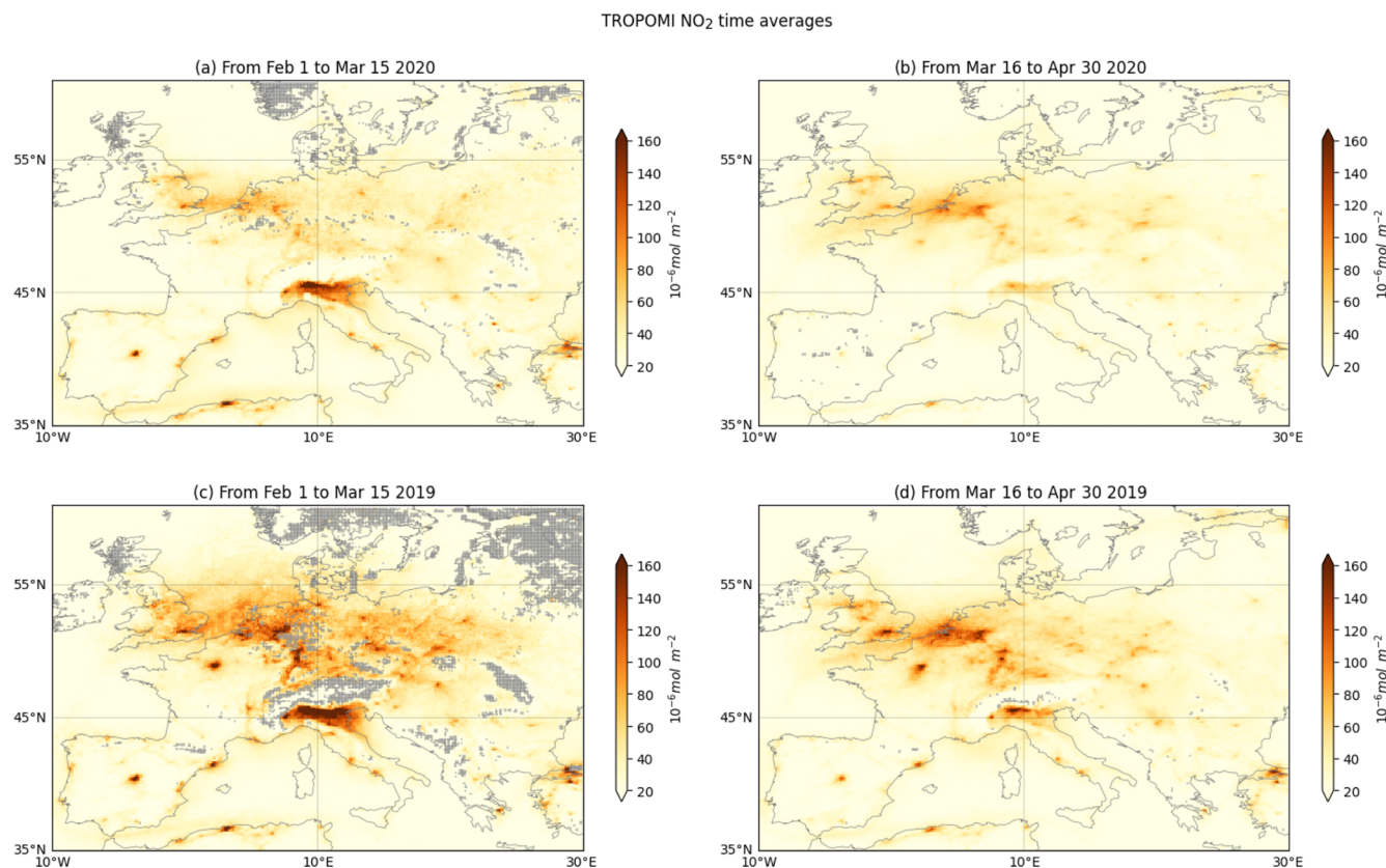
Figure 1. Average maps of the TROPOMI NO 2 tropospheric columns ( \text{mol m}^{-2} ) for European pre-lockdown and lockdown periods in 2020 (a, b) and corresponding periods in 2019 (c, d). Grey areas indicate where the number of revisits is strictly below five.
