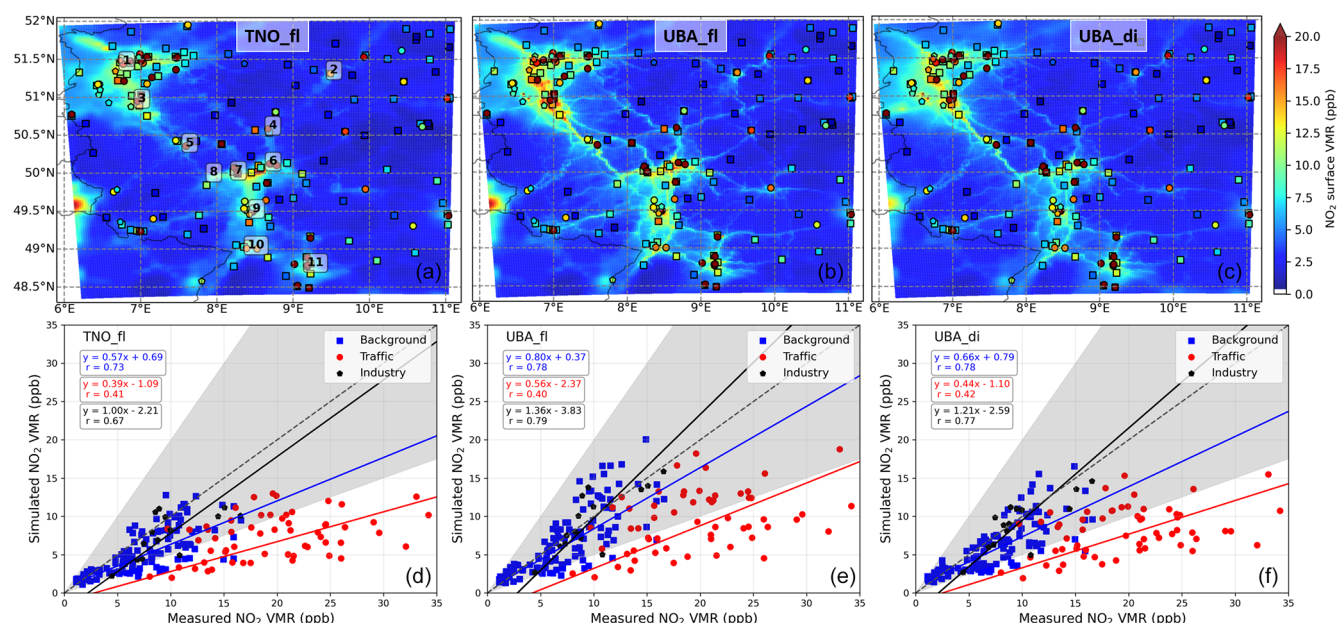
Figure 4. (a, b, c) Spatial distribution of monthly-mean NO 2 surface VMRs for the three simulations using different emission inventories (a, d: TNO, b, e: UBA without diurnal variations, c, f: UBA with diurnal variations) for CM02 for May 2018. The square, circle and pentagon markers overlaid on the maps represent the monthly-mean measured NO 2 VMRs for background, traffic and industrial locations, respectively. The numbers on the top left panel correspond to the following German cities in decreasing order of latitude coordinate values, i.e. 1: Duisburg, 2: Kassel, 3: Köln, 4: Gießen, 5: Koblenz, 6: Frankfurt, 7: Mainz, 8: Bingen, 9: Mannheim, 10: Karlsruhe 11: Stuttgart. (d, e, f) Scatter plot and orthogonal distance regression weighted by the inverse of the square of the standard deviation of simulated monthly-mean NO 2 surface VMRs with respect to the in situ measured values for different station types (background: blue square; traffic: red circle, and industrial: black pentagon).
