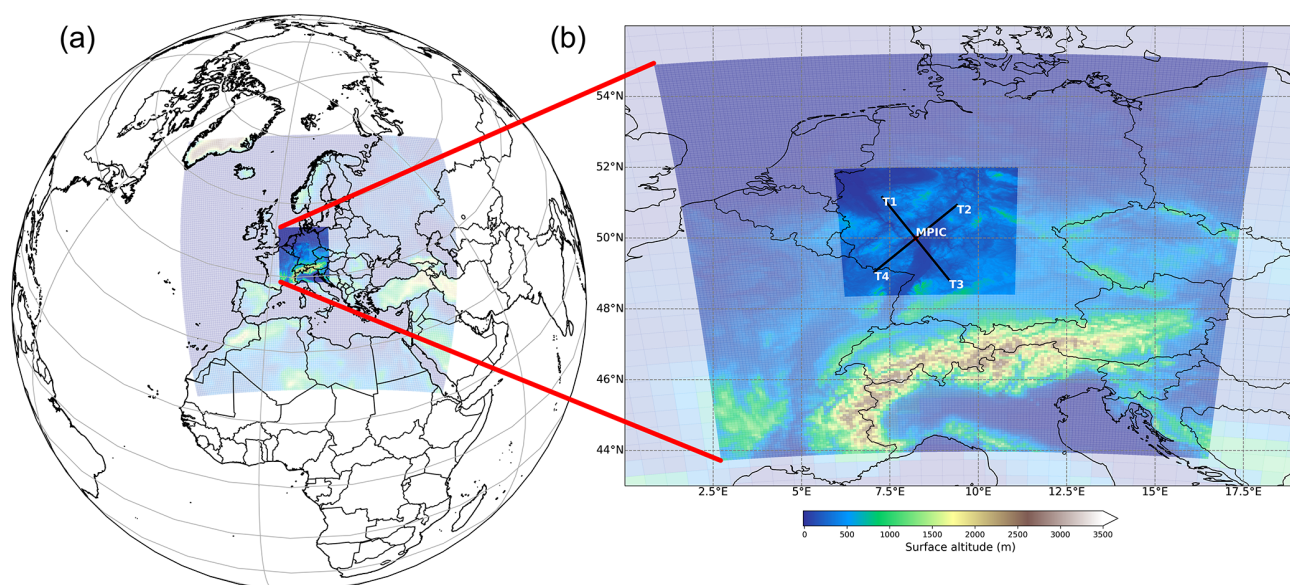
Figure 1. MECO(3) domains in panel (a) colour-coded according to the surface altitude. A close-up of the map in the right panel shows the CM07 and CM02 domains. The location of MPIC (Max Planck Institute for Chemistry) is shown as the red dot in panel (b) with the arrows pointing in the viewing direction of the four telescopes.
