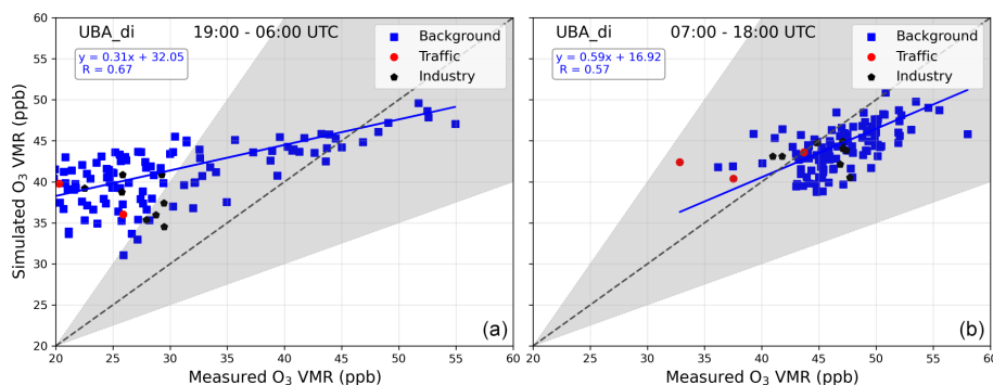
Figure B2. Scatter plot between measured and simulated \text{O}_3 for night-time ( a ) and daytime ( b ) for monthly means at all the measurement stations in the CM02 domain for the \text{UBA}_{\text{di}} set-up.
