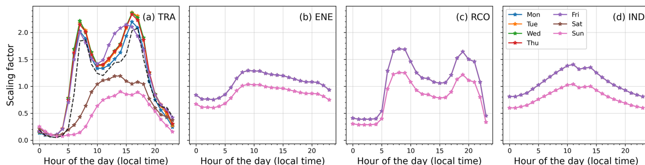
Figure A1. Temporal profiles of NO x emissions from various sectors. “TRA”: road transport, “ENE”: energy generation, “RCO”: residential and non-industrial combustion, “IND”: industries. For TRA, lines and markers correspond to the profiles derived using actual vehicle count, while for others profiles are derived according to the recommendation of Schaap et al. (2005). For TRA, the recommendations of Schaap et al. (2005) are shown as the dashed line in panel (a).
