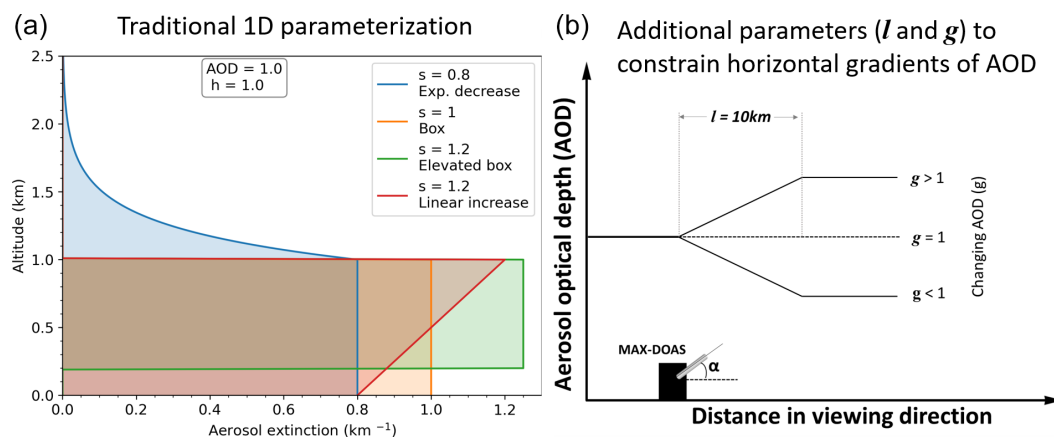
Figure 2. (a) Schematic illustration of traditional 1D parameterized profile inversion which constrains AOD, height ( h ) and shape ( s ) of the profile. The example shown here corresponds to a scenario with \text{AOD} = 1.0 , h = 1.0 and four different profile shapes representing exponential decrease, box profile, elevated box profile and linearly increasing profiles. (b) Additional parameters l and g further constrain the horizontal gradients of AOD for 2D profile inversion. Here, g denotes a linear change in AOD for a distance l along the viewing direction of the MAX-DOAS instrument.
