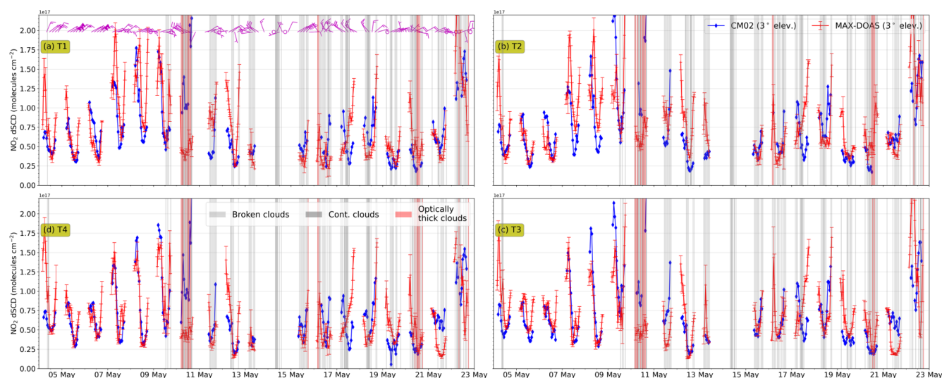
Figure 11. Same as Fig. 9 but for 3° elevation angle.
