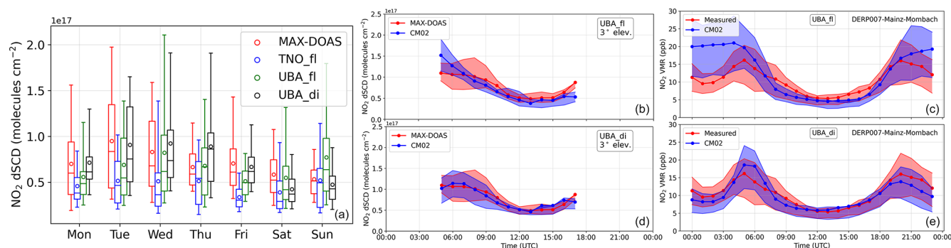
Figure 13. (a) Box and whiskers plot showing the distribution of NO 2 dSCDs at 3° elevation angles for MAX-DOAS and the three different model set-ups for different days of the week. Mean hourly diurnal profiles of measured and simulated NO 2 dSCDs at 3° elevation angle for T1 for the UBA fl (b) and UBA d1 (d) set-ups. The shaded region above and below the mean line denote the 75th and 25th percentiles, respectively. Diurnal profiles of measured and simulated NO 2 surface VMRs measured at a background site (Mombach, ~ 3.5 km north of MPIC) for the UBA fl (c) and UBA d1 (e) simulations.
