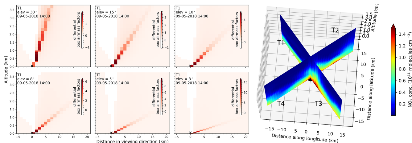
Figure 8. Left: the differential box air mass factors (dbAMFs) for 30, 15, 10, 8, 5 and 3° elevation angles retrieved using 3D profile inversion of measured O 4 dSCDs along the direction of telescope T1. Please note the different colour scales of differential dbAMFs used for the different elevation angles. Right: simulated NO 2 concentrations from the UBA di set-up in the CM02 domain from surface up to an altitude of 2.5 km along the viewing directions of the four telescopes T1, T2, T3 and T4 on 9 May 2018 14:00 UTC.
