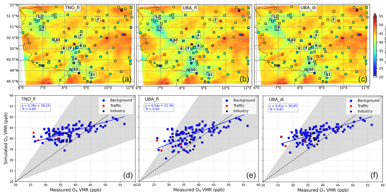
Figure B1. Spatial distribution of monthly-mean \text{O}_3 surface VMRs for the three simulations using different emission inventories ( a , d : TNO, b , e : UBA without diurnal variations, c , f : UBA with diurnal variations) for May 2018. Panels ( d ), ( e ) and ( f ) show the scatter plot and orthogonal distance regression (ODR) weighted by the inverse of the square of the standard deviation of simulated monthly-mean \text{O}_3 surface VMRs with respect to the in situ measured values. ODR was performed only for the background stations because of the low number of stations at the traffic-adjacent and industrial locations.
