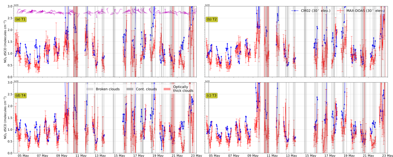
Figure 9. Comparison of \text{NO}_2 differential slant column densities at 30^\circ elevation angle of the four telescopes simulated using \text{UBA}_{\text{di}} in the CM02 domain. The shaded regions in the time series represent various categories of sky conditions as described in the legend.
