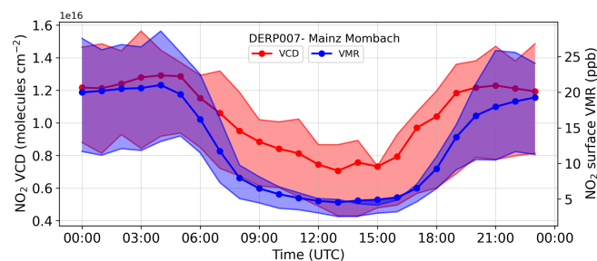
Figure C4. Mean hourly diurnal profiles of simulated NO 2 tropospheric VCDs (red) and surface volume mixing ratios (blue) at a background site (Mainz Mombach; 8.02° E, 50.02° N) for the model set-up UBA fl (diurnal variability of road transport and non-industrial combustion sectors not considered). The solid line and markers represent the mean, while the shaded region shows the inter-quartile variability range.
