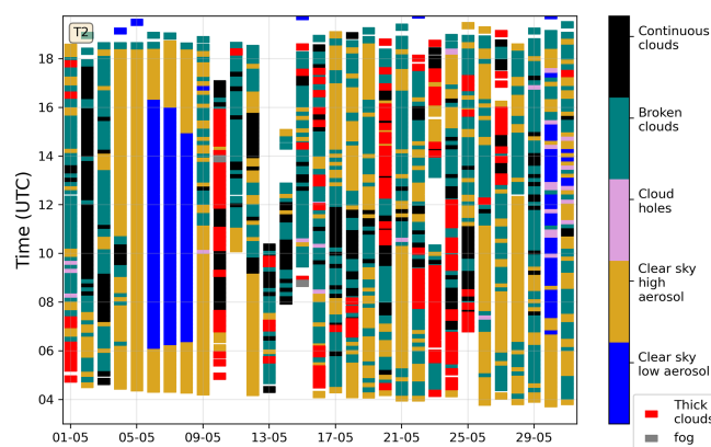
Figure C1. Daily variability of the sky conditions for May 2018 retrieved using MAX-DOAS measurements along the azimuth direction of T2. Consistent sky conditions were retrieved for the other three azimuth directions
