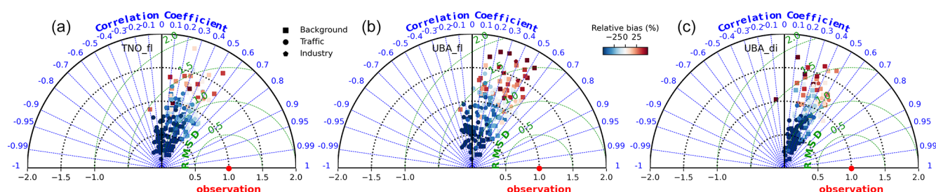
Figure 5. Taylor diagrams showing the Pearson correlation coefficients, normalized standard deviation and normalized root mean square difference corresponding to hourly resolution measured and simulated \text{NO}_2 VMRs (in CM02 domain) for background, traffic and industrial sites represented as square, circle and pentagon markers, respectively. Panels (a), (b) and (c) correspond to the \text{TNO}_{\text{fi}} , \text{UBA}_{\text{fi}} and \text{UBA}_{\text{di}} set-ups, respectively.
