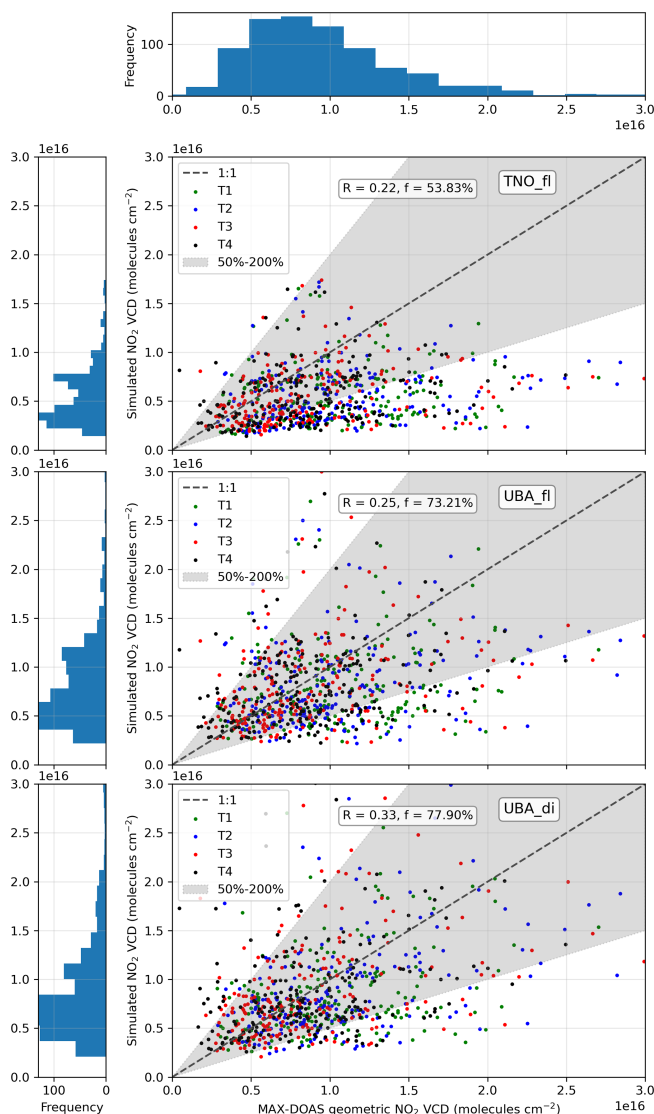
Figure 7. Scatter plot of simulated VCDs against measured VCDs for all four telescopes combined for 30° elevation angle. Individual points correspond to the hourly-mean VCD values. The top, middle and bottom panels correspond to TNO fl , UBA fl and UBA di , respectively. R represents the Pearson correlation coefficient, and f represents the fraction of simulated NO 2 VCDs no less than half and no greater than twice the magnitude of geometric VCDs. The frequency distribution of the measured VCDs is shown above the first panel, and those for the simulated VCDs from the three set-ups are shown on the left of the respective scatter plots.
