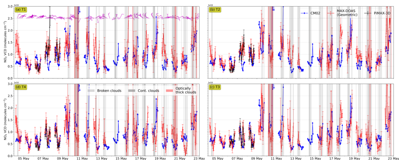
Figure 6. Comparison of \text{NO}_2 VCDs along the viewing directions of the four telescopes (T1–T4) simulated using the \text{UBA}_{\text{di}} set-up in the CM02 domain. MAX-DOAS VCDs are retrieved using geometric approximation (red markers) for the complete measurement period and using \pi -MAX for 3 d (black markers). The error bars represent the hourly 1\sigma standard deviations. The shaded regions in the time series represent various categories of clouds as described in the legend. The purple bars in panel (a) show the measured wind speed and wind directions, with half arrows, full arrows and flags corresponding to wind speeds of 1, 2 and 5 \text{ m s}^{-1} , respectively.
