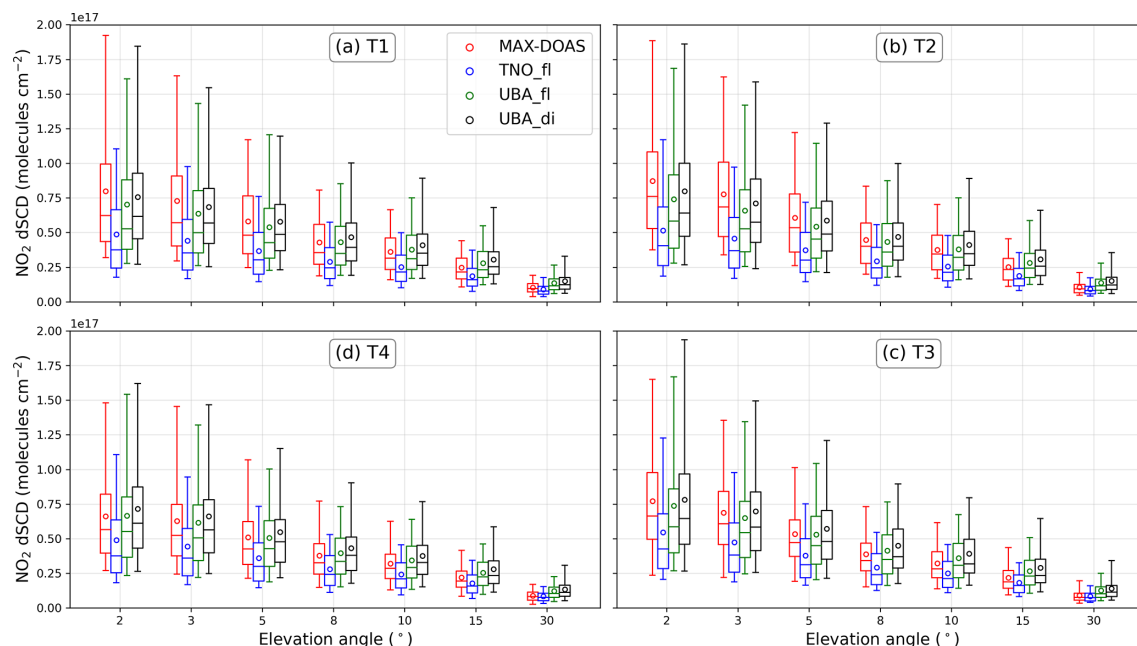
Figure 10. Box and whiskers plots for the different telescopes (a–d) showing the distribution of measured and simulated dSCDs for the three different model set-ups (depicted in different colours) for various elevation angles (2, 3, 5, 8, 10, 15, and 30^\circ ).
