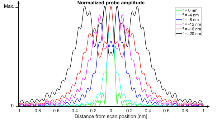
Figure 14: Profiles of the electron probe wave function (amplitude normalised to its maximum) in dependence of focus for 200 kV electrons and a semi-convergence angle of 23 mrad. Even for comparably large foci, the full width at half maximum is still within the range of 1 nm.
