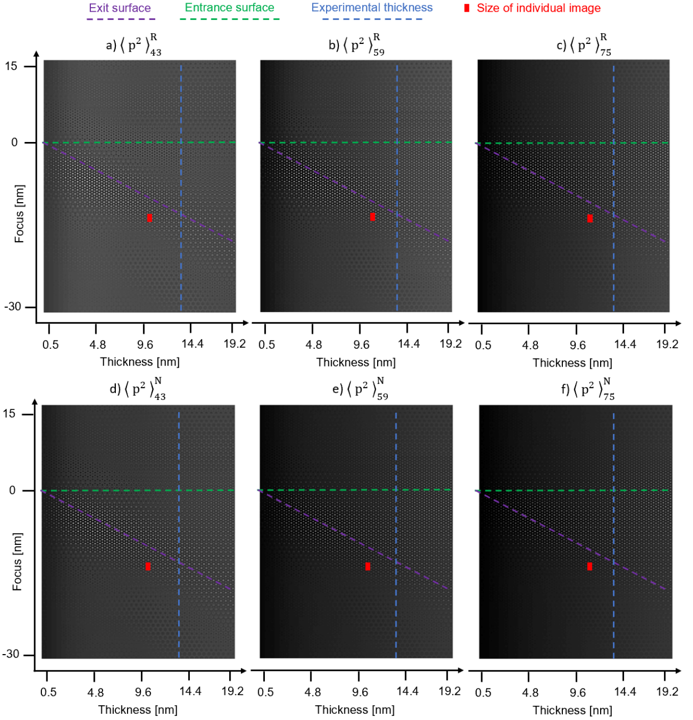
Figure 11: \langle p^2 \rangle^R_{\theta_l} and \langle p^2 \rangle^N_{\theta_l} signals for increasing cut-off angles \theta_l . Data is given as a function of specimen thickness and probe focus, the latter being zero at the entrance surface. The positions of the entrance and exit surfaces on the focus axis are indicated as well. The size of an single image in the graph is indicated as a red rectangle.
