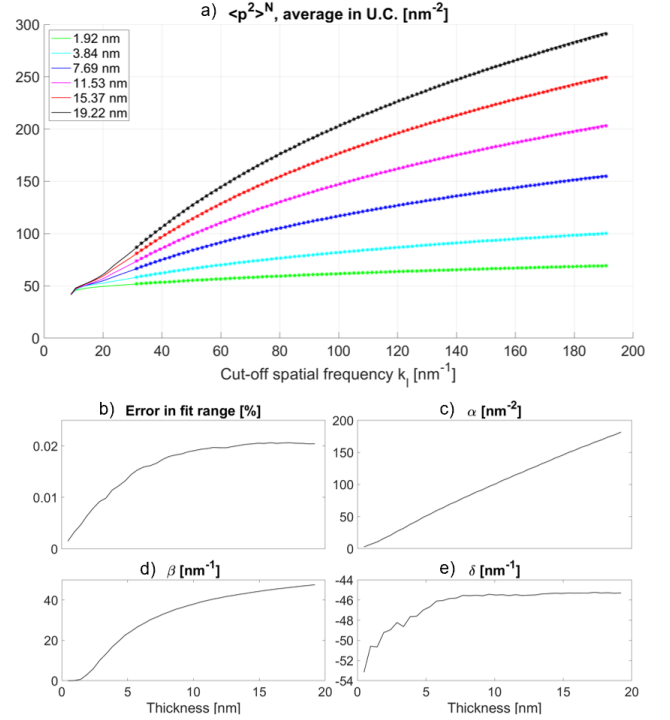
Figure 13: a) Results of the real-space average of \langle p^2 \rangle_{\theta_l}^N images, within one unit cell, for increasing cut-off frequencies k_l . The measurement is done with varying thickness, and a focus equal to zero. The curves are fitted with a parametric function, depicted as dot curves. b) Values taken by the fitting parameters \alpha , \beta and \delta , as well as the average quadratic error within the considered range, plotted as functions of thickness.
