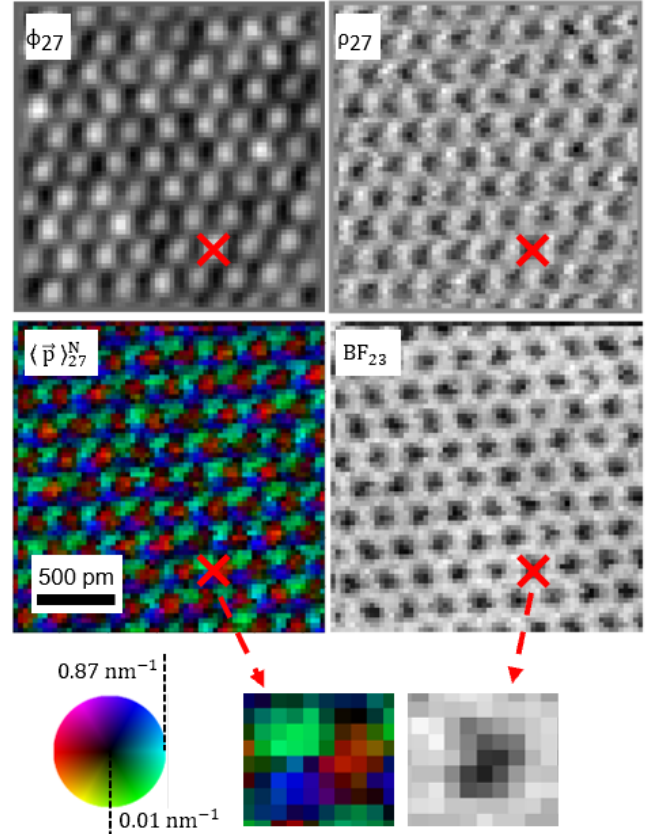
Figure 6: The \langle \vec{p} \rangle_{27}^N vector field, at its focus of maximum contrast, is displayed alongside its divergence and integral. The BF 23 counterpart is depicted as well. A subset of the images is shown containing the expected atomic pattern, meaning a set of first moment vectors pointing toward the atomic site.
