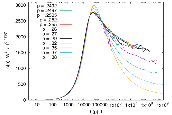
FIG. 10. Same data as in Fig. 9, but curves are shifted horizontally and vertically, and divided by t^{2\beta_{\text{KPZ}}} . Plotted in this way it becomes obvious that systems are too small for p < 0.251 to show a possible KPZ scaling, while t is too small for p > 0.28 .
