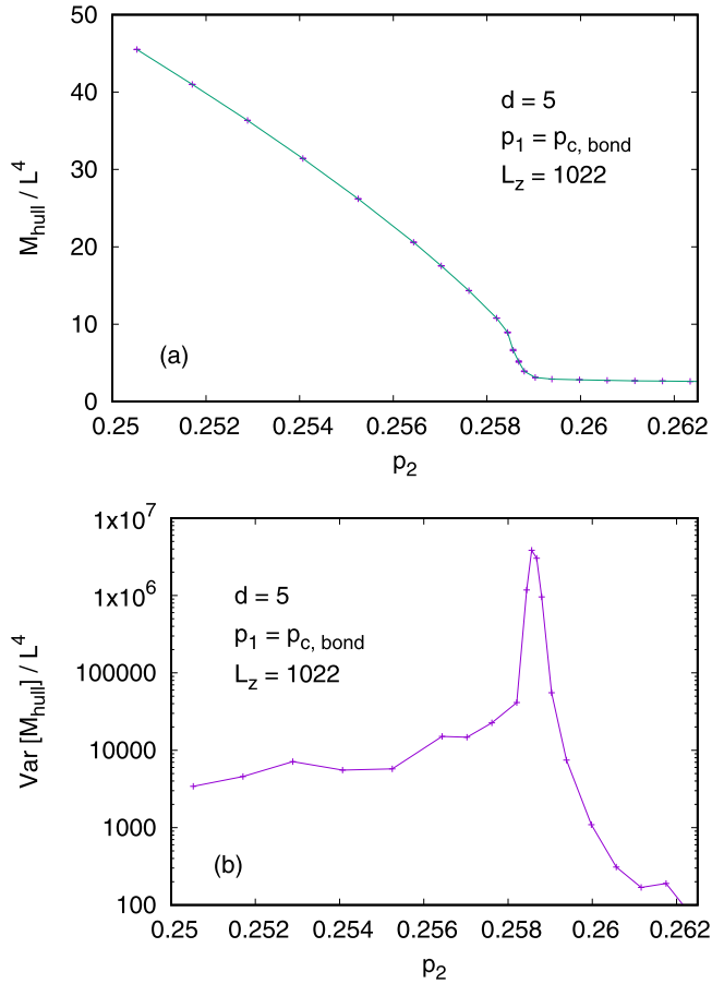
FIG. 2. (a) Mass density (per unit base surface) of the external hull of the cluster growing upwards from z = 0 in dimension D = 5 and at p_1 = p_{c, \text{bond}} . This density would be infinite in the sponge phase, if the cluster thickness L_z were infinite. Panel (b) shows the variance of the mass density.
