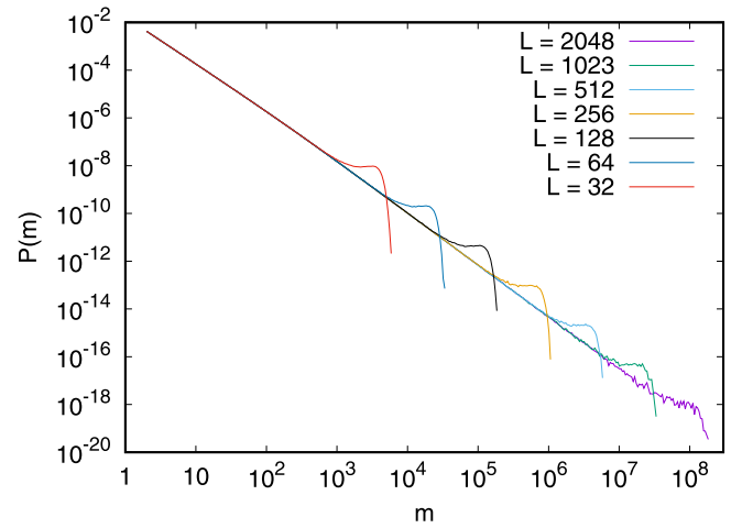
FIG. 3. Mass distribution of clusters inside the holes of the giant cluster in supercritical bond percolation in D = 3 , with p = p_{b, \text{sponge}} = 0.31958 chosen such that the holes just contain a incident giant cluster (notice that this second cluster is grown with p = 1 , i.e., we are at the threshold where a giant cluster exists in the complement of the first cluster). As in ordinary 3-D percolation, we have P(m) \sim m^{-\tau} with \tau = 2.189 in the scaling region and a peak position scaling m_{\text{max}} \sim L^{D_f} with D_f = 2.523 .
