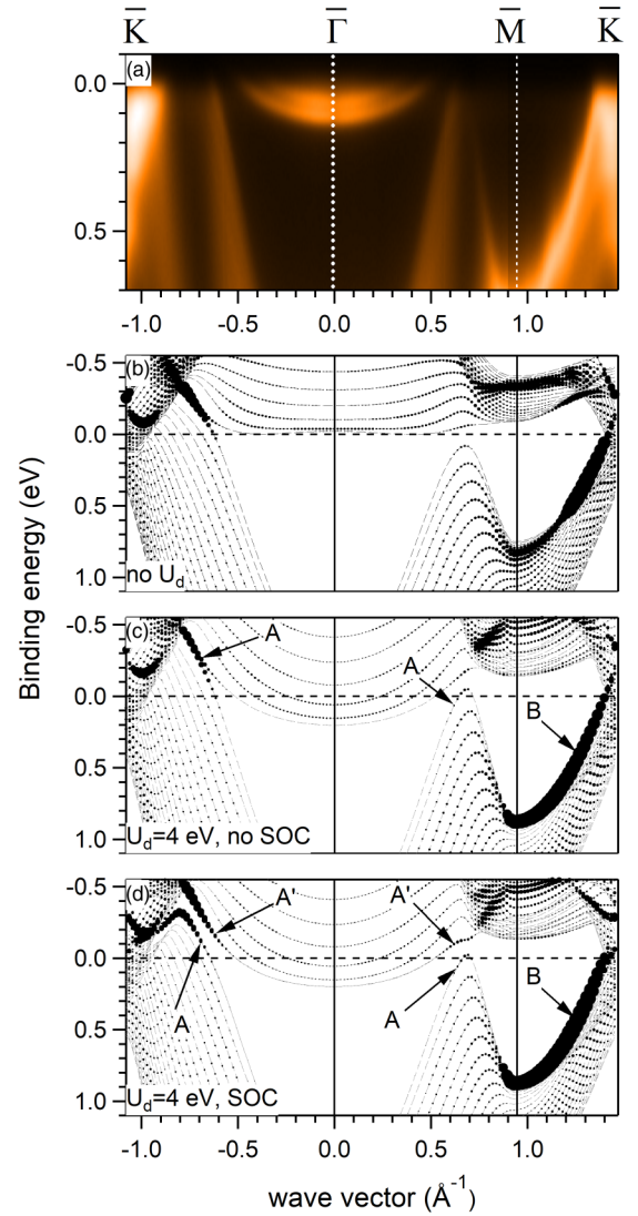
FIG. 2. (a) Photoemission intensity map along the \bar{K}\bar{\Gamma}\bar{M}\bar{K} of a 29-ML Yb film for h\nu = 34 eV; (b),(c) Calculated surface band structure of 24-ML Yb(0001) film; symbol size is proportional to the s + p + d character in the top two layers. (b) Without U_d , no SOC; (c) with U_d = 4 eV, no SOC; (d) with U_d = 4 eV, SOC. Black arrows indicate the surface states A, A', and B.
