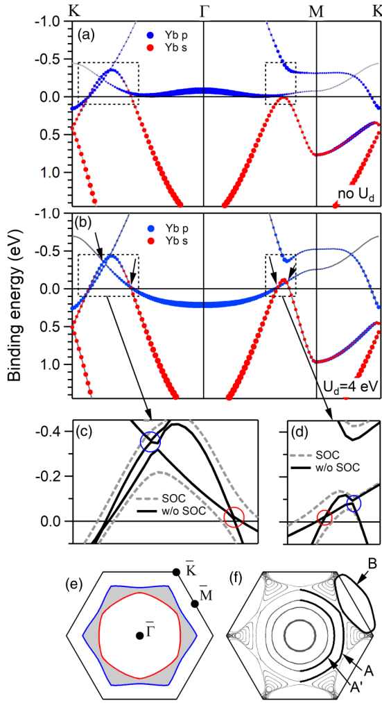
FIG. 3. (a),(b) DFT bulk band structure of hcp Yb along K\Gamma MK with orbital projections without SOC (a) without U_d and (b) with U_d = 4 eV. (c),(d) Zooms on the band crossing without (black solid) and with (gray dashed) SOC included. Red (blue) circles indicate band crossings with an integral of the Berry curvature around the nodal line corresponding to -\pi ( +\pi ). (e) Surface Brillouin zone with a shaded region indicating the k_{\parallel} distribution of the \pi Zak phase. (f) DFT + U_d constant energy cut taken at Fermi level for a 24-ML film with SOC included corresponding to the same slab with surface band structure shown in Fig. 2(d). Thicker lines mark the surface states A , A' , and B .
