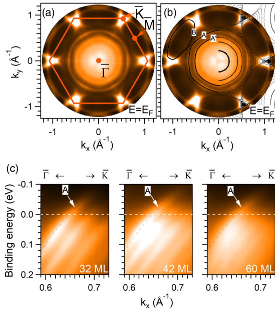
FIG. 4. (a) Constant energy cuts on a 29-ML Yb film with 34 eV photon energy taken at E_F . (b) The same, overlapped with DFT calculated Fermi surface from Fig. 3(f). (c) ARPES maps along the \bar{\Gamma} - \bar{K} direction for different thicknesses as indicated, with photon energy 9 eV. The dashed lines are guides to the eye.
