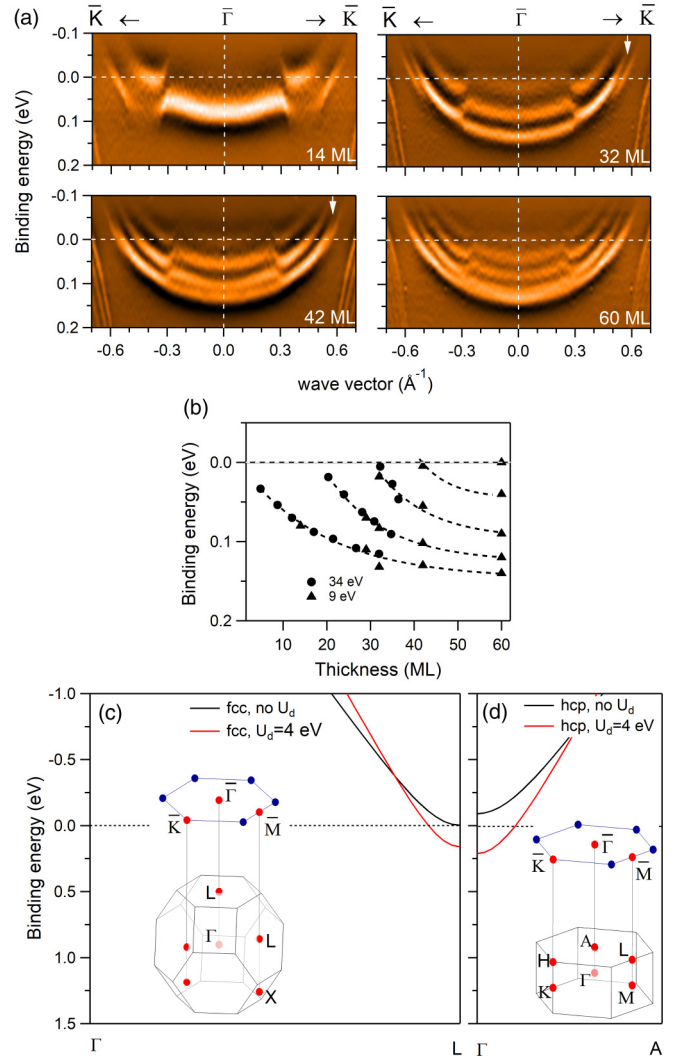
FIG. 1. (a) ARPES maps taken with h\nu = 9 eV at room temperature along \bar{K} \bar{\Gamma} \bar{K} direction and around E_F for different thicknesses as indicated. The images are taken around the \bar{\Gamma} point, normalized to the Fermi function and in a form of second derivative. (b) Energy position versus film thickness of the bands at the \bar{\Gamma} point represented by solid symbols (circles for the experiment obtained at h\nu = 34 eV and triangles for experiments obtained at h\nu = 9 eV); the dashed lines are a guide to the eye. (c) Theoretical bulk band dispersion without SOC effects along the \Gamma L high-symmetry line of the fcc structure. The inset shows the correspondence of the bulk and surface fcc Brillouin zones. (d) Theoretical bulk band dispersion without SOC effects along the \Gamma A high-symmetry line of hcp structure. The inset shows the correspondence of the bulk and surface hcp Brillouin zones.
