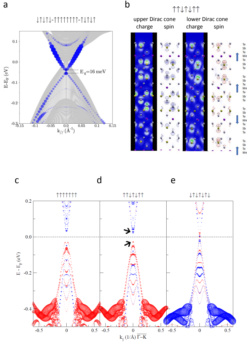
FIG. 16: Influence of magnetic structure on topological surface states (DFT). (a) Band structure for a ferromagnetic bulk surrounded by antiferromagnetic surface layers as marked on top. Blue dots are surface states with dot diameter marking their strength at the surface septuple layer. A gap appears in the topological surface state. (b) Charge density and spin density of the states at the edges of the magnetically induced band gap in (d) displayed as thin film cross section. The magnetic configuration is marked on top. (c–e) Band structure for various magnetic configurations each marked on top. Colors denote the spin density in the out-of-plane direction. (c) Ferromagnetic order with out-of-plane anisotropy. (d) Two ferromagnetic septuple layers on both sides of three antiferromagnetic layers. Black arrows mark the states shown in (b). (e) Perfect antiferromagnetic order as in Fig. 4d,e, main text.
