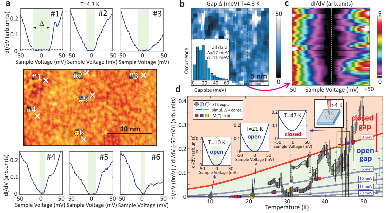
FIG. 3: Spatial variation of the magnetic energy gap and closing at T_C . (a) Center: STM image of MnSb 2 Te 4 after UHV transfer from the MBE, V = 0.5 V, I = 0.2 nA, T = 4.3 K. Surrounding: dI/dV spectra recorded at the labelled crosses. Dashed line in the upper left spectrum: noise threshold used for determination of gap size \Delta (Supplementary Section IX). (b) Spatial map of gap size \Delta . Inset: histogram of \Delta resulting from three distinct areas, average gap size \bar{\Delta} and standard deviation \sigma are marked. (c) dI/dV spectra (color code) along the magenta dashed line in (b). Yellow line at the bottom of the color code bar: threshold for gap determination in (a,b). (d) Small dots: Ratio R = [dI/dV(V=0 \text{ mV})] / [dI/dV(V=-50 \text{ mV})] deduced from dI/dV(V) curves at different T . Different grey shades: different cooling cycles. Each point belongs to a single position on the sample surface within 1 nm. Error bars: standard deviation resulting from multiple curves measured at the same position. Large grey dots: average values at the corresponding T representing spatially averaged gap sizes \bar{\Delta}(21 \text{ K}) = 11 \pm 5 meV, \bar{\Delta}(31 \text{ K}) = 6 \pm 1 meV, and \bar{\Delta}(36 \text{ K}) = 4 \pm 1 meV (Supplementary Section IX). Grey lines: T -dependence of the ratio R for the marked gap sizes \bar{\Delta} , deduced by convolving the measured dI/dV(V) at 4.3 K with the Fermi distribution (Supplement: Fig. 13b). The area above \Delta = 0 meV exhibits such a large R that the existence of a gap is excluded. Error bars on the right mark a standard deviation due to variation of the dI/dV curves at 4.3 K (Supplement: Fig. 13b). Colored squares: gap values deduced from XMCD (yellow, Fig. 1f) and SQUID (red, violet, Supplement: Fig. 7) using \bar{\Delta}(T) \propto M(T) [70]. Insets: selected dI/dV curves for the points with blue arrows. Additional curves: Supplement: Fig. 12
