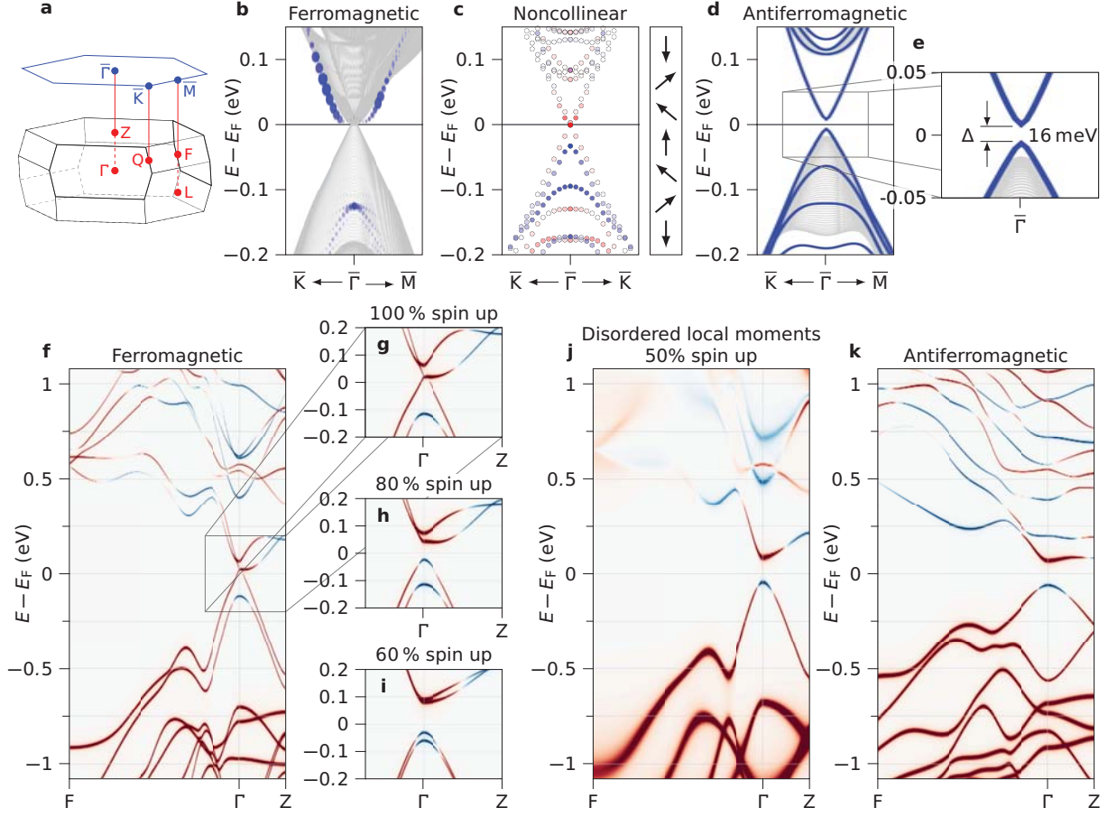
FIG. 4: Theoretical predictions for MnSb 2 Te 4 . (a) Brillouin zone of bulk (bottom) and surface (top) of MnSb 2 Te 4 with marked high symmetry points. (b-e) Band structures from DFT calculations of slab geometries for various magnetic configurations (marked on top). (b) Ferromagnetic interlayer coupling for a thick slab. Blue dots: surface states identified via their strength in the top septuple layer. (c) Non-collinear interlayer coupling (sketched on the right) for a thin slab. Color code: out-of-plane spin polarization of the gapped Dirac cone. Uncolored circles: bulk states. (d) Antiferromagnetic interlayer coupling for a slab (blue lines) on top of the projected bulk band structure (grey lines) with a gapped Dirac cone at \bar{\Gamma} . (e) Zoom into (d) with marked magnetic gap size of the topological surface state. (f-k) Band structures from DFT calculation for a bulk geometry with magnetic configurations as marked on top. Red (blue): dominating anion (cation) character as spectral function difference between anion and cation sites for each state (Supplementary Section XI). (f) Ferromagnetic interlayer coupling with a topologically protected Weyl cone around \Gamma . (g) Zoom into (f). (h,i) same as (g) but with magnetic disorder modelled via overlap of collinear spin up and spin down states at each Mn site (Supplementary Section XI). (j) Same as (f), but with full magnetic disorder. (k) Antiferromagnetic interlayer coupling. An inverted band gap appears for (h-k) at \Gamma around E_F visible by the exchanged colors of the two bands, i.e., these structures are topological insulators.
