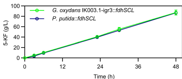
Fig. 3. Biotransformation of fructose to 5-KF with resting cells. Cell suspensions of G. oxydans IK003.1-igr3:: fdhSCL and P. putida::fdhSCL at an OD 600 of 3 were incubated in 100 mM potassium phosphate buffer pH 6 with 150 g l -1 fructose at 30°C and 180 rpm. 5-KF concentrations were determined by HPLC. Mean values and standard deviations of biological triplicates are shown.
