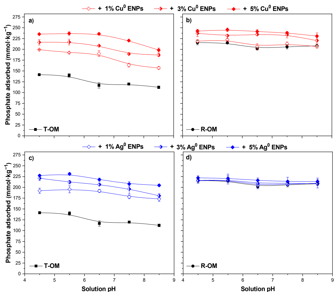
Figure 2. Initial pH effect of the solution on the adsorption of \text{H}_2\text{PO}_4^- in the presence of \text{Cu}^0 ENPs on soil with (a) total organic matter (T-OM) and (b) partial removal of organic matter (R-OM) and \text{Ag}^0 ENPs on soil with (c) T-OM and (d) R-OM.
