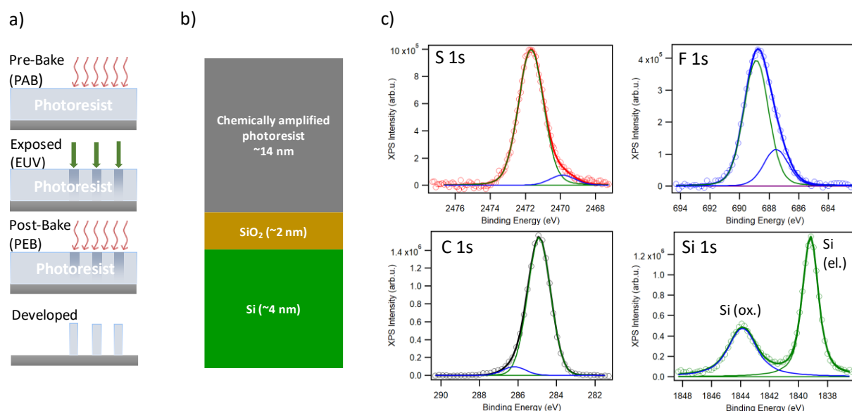
Figure 2. a) Schematic of chemically amplified resist (CAR) processing b) Sample schematics including expected/nominal layers' respective thicknesses c) Core levels XPS spectra of the PAB-CAR (S 1s, F 1s, C 1s) and Si 1s from the substrate, exhibiting elemental and oxidized species.
