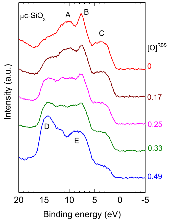
Fig. 4. Experimental HAXPES valence band spectra of \mu\text{c-SiO}_x\text{:H} samples (with [\text{O}]^{\text{RBS}} = 0, 0.17, 0.25, 0.33 , and 0.49 ). Note that the spectra are offset vertically for easier comparison.
