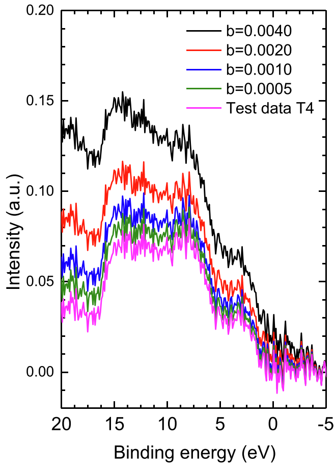
Fig. 3. Impact of the addition of linear backgrounds with different slopes ( b ) on the spectral shape of the calculated HAXPES valence band spectra (test data T4).
