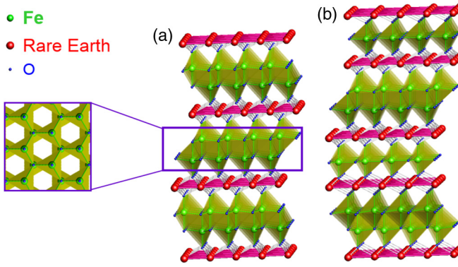
FIG. 1. Crystal structure of (a) rhombohedral \text{LuFe}_2\text{O}_4 with three Fe-O bilayers in the unit cell, and (b) hexagonal \text{Lu}_2\text{Fe}_3\text{O}_7 with two Fe-O bilayers and one monolayer in the unit cell. The inset shows the projection of one bilayer in the ab plane.
