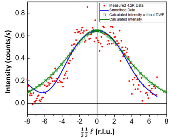
FIG. 8. Diffuse magnetic scattering at the (\frac{1}{3}\frac{1}{3}\ell) line (intensity averaged along hh0 from 0.25 to 0.4) in the spin-flip channel for neutron polarization parallel to \vec{z} direction at 4.2 K. The smoothed data (blue) and the intensity model for the random distribution of \text{Fe}^{2+} and \text{Fe}^{3+} (green line, squares: with, without Debye-Waller factor) are also shown. Background is subtracted for the measured data.
