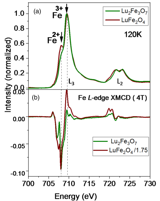
FIG. 10. (a) XAS spectrum [ \text{XAS} = (\mu_- + \mu_+)/2 ] of stoichiometric \text{Lu}_2\text{Fe}_3\text{O}_7 and \text{LuFe}_2\text{O}_4 crystals in a field of 4 T normalized to the peak maximum. (b) The corresponding XMCD signals [ \text{XMCD} = (\mu_+ - \mu_-) ]. The \text{LuFe}_2\text{O}_4 XMCD signal was taken from [18] and scaled through division by 1.75.
