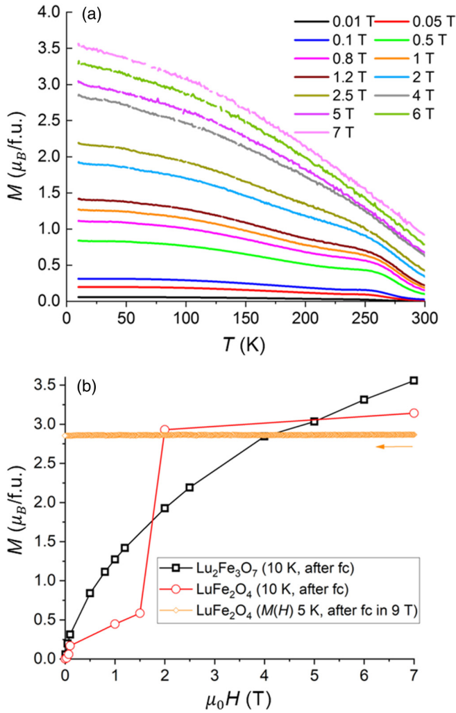
FIG. 3. (a) Temperature-dependent magnetization during field cooling and followed by field warming at different magnetic fields for SC3. FC, and FW perfectly overlap for all used fields. (b) Low-temperature magnetization obtained by cooling in different magnetic fields for \text{Lu}_2\text{Fe}_3\text{O}_7 (squares) and for \text{LuFe}_2\text{O}_4 (circles). For \text{LuFe}_2\text{O}_4 also shown (small diamonds) is M(H) obtained in decreasing H after cooling in 9 T (taken from the full M(H) loop shown in Fig. 4.5(b) in [18]).
