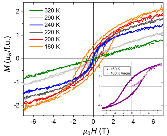
FIG. 4. M(H \parallel c) loops measured on SC3 at different temperatures. Inset: Hysteresis loop including the virgin curve measured after cooling in zero field at 160 K.
