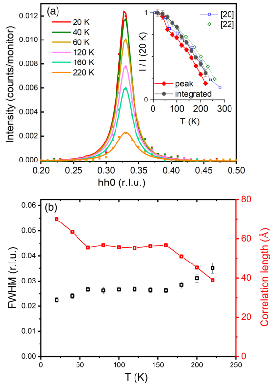
FIG. 9. (a) Diffuse magnetic scattering averaged along the \ell direction in the range \ell = -5 to \ell = 5 in the spin-flip channel measured with \vec{P} \parallel \vec{Q}_{\text{average}} vs hh0 for selected temperatures. The data were fitted with a Lorentzian (solid curves) and the background is subtracted for all curves. The inset shows the temperature dependence of both integrated and peak intensities. The peak intensities of [20,22] are also shown for comparison. (b) Correlation length and full widths at half maxima extracted from the data fitting for various temperatures.
