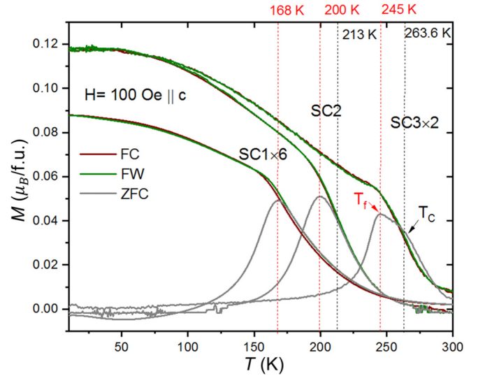
FIG. 2. Temperature dependence of magnetization measured with a field of 100 Oe applied parallel to the c direction during cooling (FC), warming (FW), and warming after zero-field cooling (ZFC) in a temperature range of 10–300 K for different \text{Lu}_2\text{Fe}_3\text{O}_7 single crystals. SC1 and SC3 are scaled for better visibility. T_c is assigned by the steepest slope in the FC curve, T_f by the maximum of the ZFC curve.
