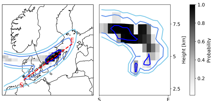
Figure 11. Probability maps on 16 April 2010, 00 UTC, from the 24 h assimilation window test case. a) Probability of the analysis ensemble for volcanic ash column mass loading exceeding 2 \text{ gm}^{-2} . Contour lines of nature run volcanic ash column mass loading for 0.5, 1, and 2 \text{ mgm}^{-2} are also given by blue lines. b) Probability of the analysis ensemble of volcanic ash concentration exceeding 500 \text{ µgm}^{-3} along the red dashed line in a). Contour lines of nature run volcanic ash concentrations for 250, 350, and 500 \text{ µgm}^{-3} are shown by blue lines.
