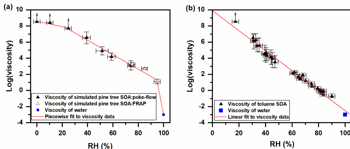
Figure 1. Panel a shows the log(viscosity) data from Smith et al. 55 as a function of the activity of water (RHs < 50%) and new measurements (RHs > 50%) using poke-flow and fluorescence recovery after photobleaching (FRAP) (Section S1 and S2) for simulated pine tree SOA, the viscosity of pure water, as well as a fit to the data using eq 1-3. Panel b shows the log(viscosity) data from Song et al. 48 as a function of the activity of water for toluene SOA, the viscosity of pure water, and a fit to the data using eq 6. For both panels the x-error bars represent uncertainties in the RH measurements and the y-error bars correspond to the upper and lower limits of the viscosities. The points with upwards arrows correspond to data where only lower limits of viscosity were obtained.
