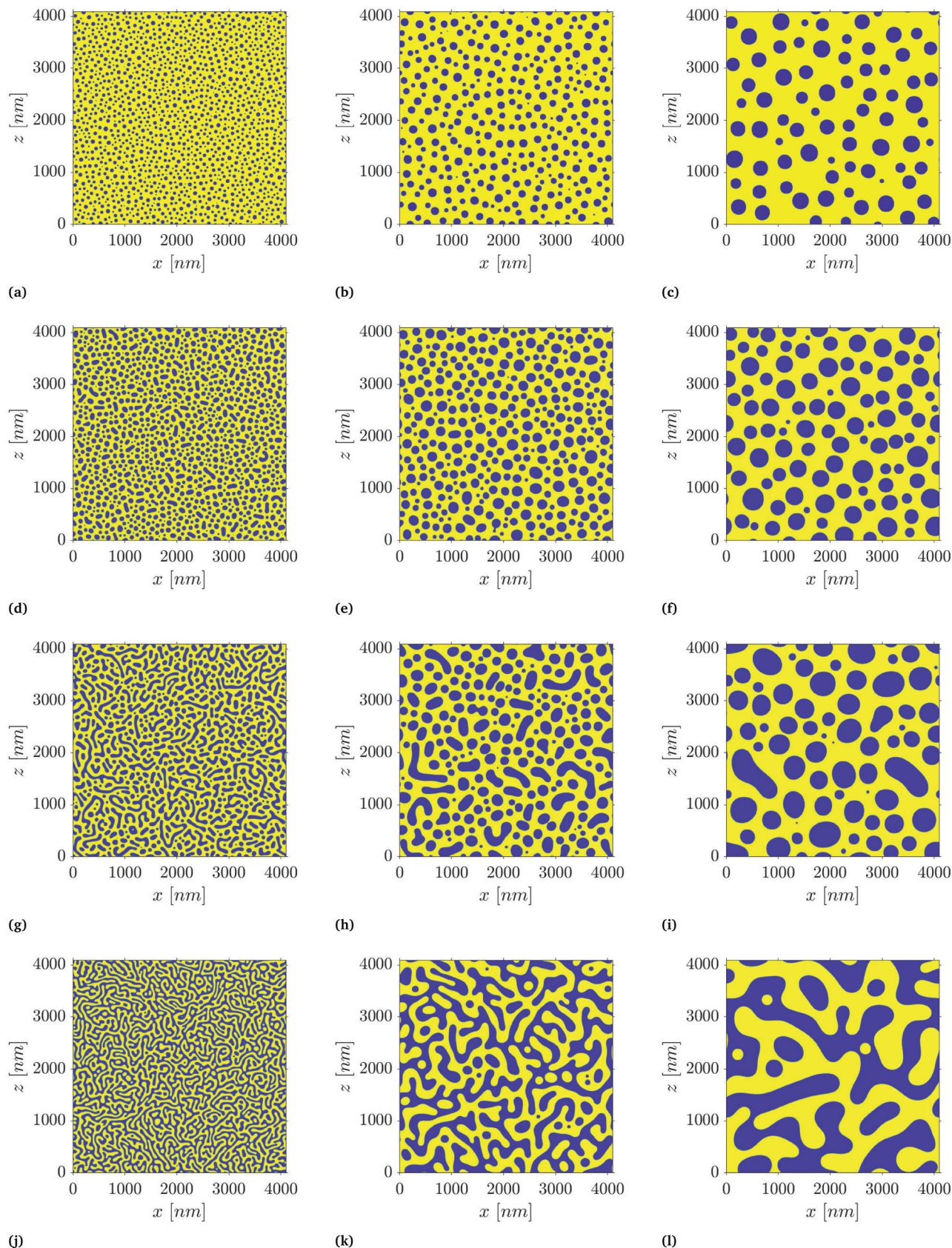
Fig. 5 Resulting morphologies for the asterisk-marked quench points in Fig. 4 for \varphi_0 = 0.25 ((a)–(c)), \varphi_0 = 0.40 ((d)–(f)), \varphi_0 = 0.45 ((g)–(i)) and \varphi_0 = 0.5 ((j)–(l)). The 1st column corresponds to 4 \times 10^{-5} s, the 2nd column to 4 \times 10^{-4} s and the 3rd one to 4 \times 10^{-3} s. For \varphi_0 = 0.25 to 0.45 , the majority concentration of the mixture constitutes the yellow matrix phase.
